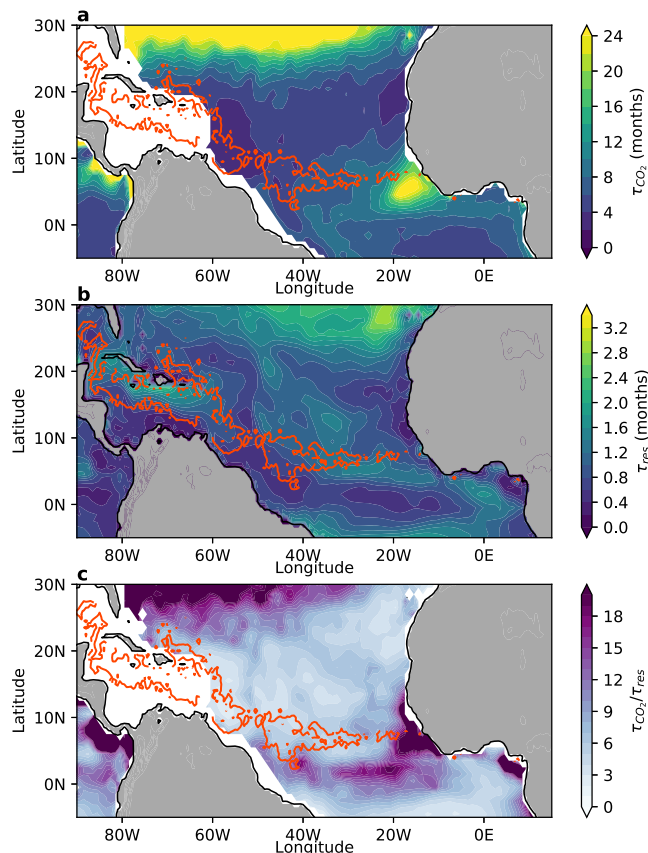
Fig. 3 Timescales of CO 2 equilibration in the Great Atlantic Sargassum Belt. The orange mask indicates the occurrence of Sargassum with >0.002 kg/m 2 during June 2018 as in Fig. 1a. a Annual mean timescales of CO 2 equilibration ( \tau_{\text{CO}_2} ) between the ocean and atmosphere. b Residence time of seawater in the surface mixed layer ( \tau_{\text{res}} ) before losing contact with the atmosphere. c Ratio of \tau_{\text{CO}_2} and \tau_{\text{res}} .
