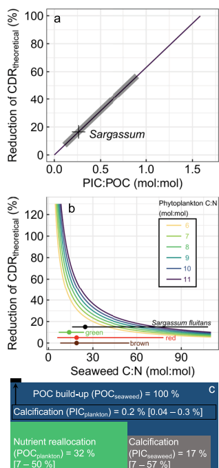
Fig. 2 Reduction of the theoretical CO 2 removal potential (CDR theoretical ) through biogeochemical feedbacks.
