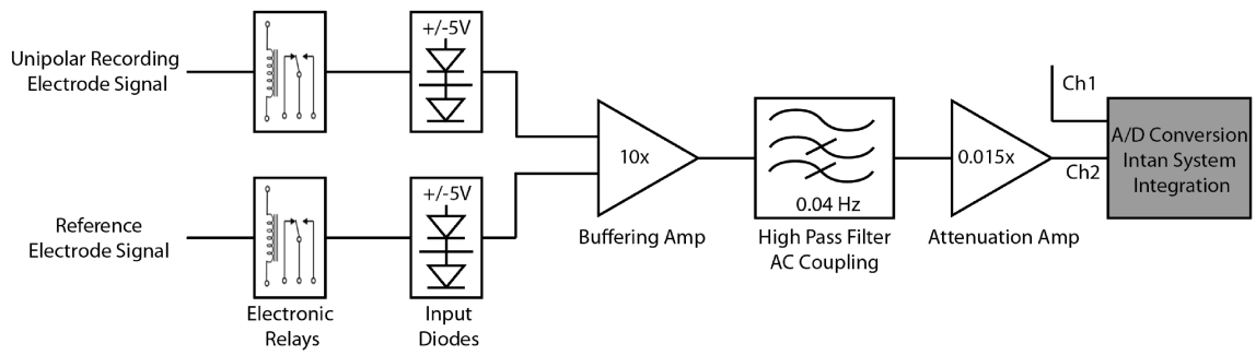
Figure 2. Block diagram of the designed front-end system including defibrillation protection (relays and diodes), filtering (high pass filter), and signal attenuation (amplifiers).
