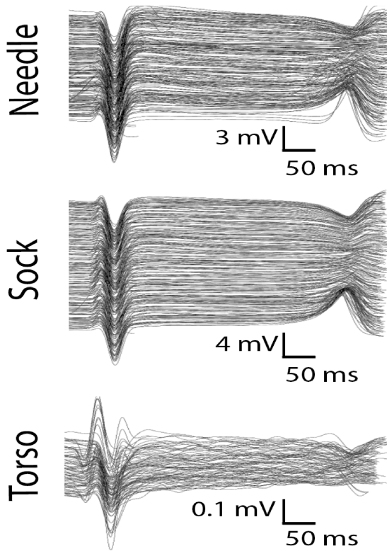
Figure 3. Example simultaneous recordings from three measurement domains: intramyocardial, epicardial, and the torso surface. A total of 530 channels are recorded from 204 needle, 233 sock, and 93 torso electrodes.
