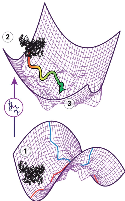
Fig. 1 Schematic view of computational studies of enzyme catalysis. An initial guess for the transition state is introduced in a crystal structure of an enzyme ①, leading to a high-energy non-equilibrium structure ② that is optimized to ③, which is assumed to represent the transition state of the reaction. Conformational changes from ② to ③ are likely to occur on the \mu\text{s} timescale and extensive sampling on the coordinates perpendicular (blue) to the reaction coordinate (red) is needed for adequate description of the transition state ensemble.
