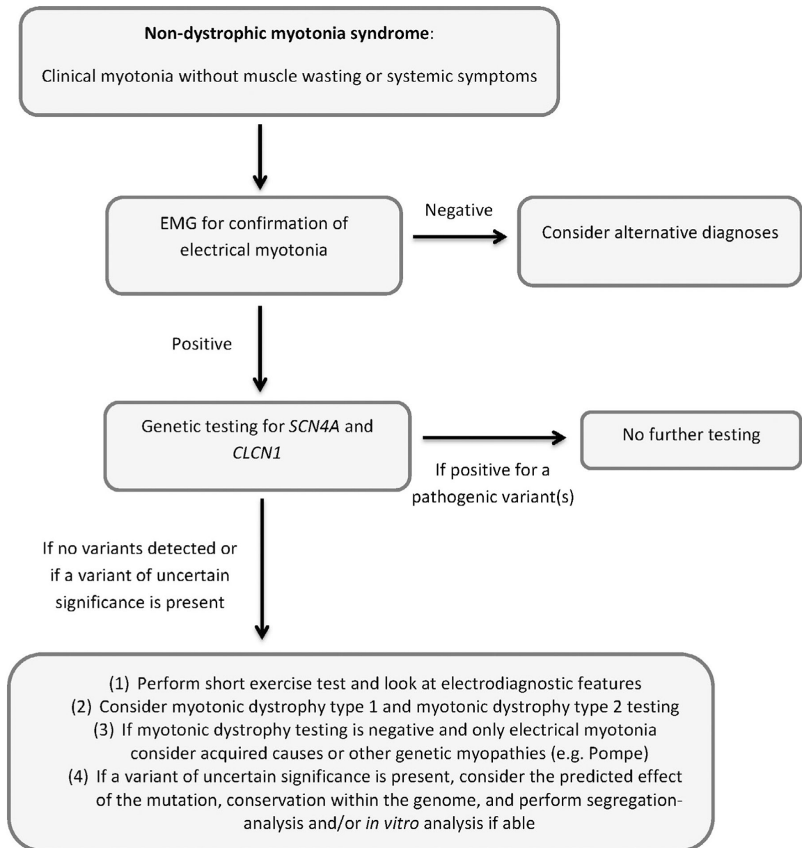
FIGURE 2. Diagnostic algorithm
