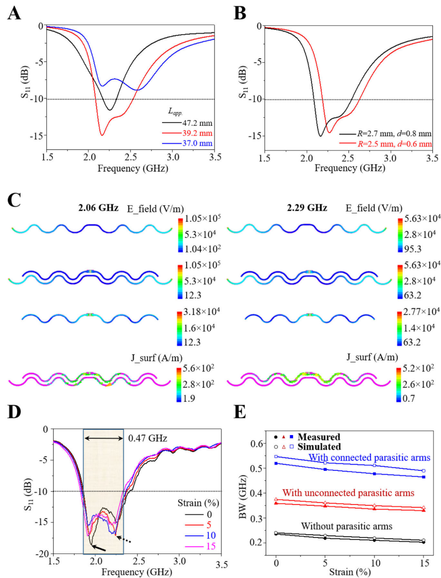
Figure 2. Design of the stretchable wideband antenna and its mechanical-electromagnetic properties.
