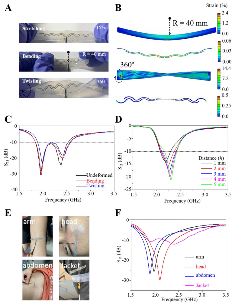
Figure 3. Characterization of the stretchable wideband antenna under large deformations or attached to human bodies.
