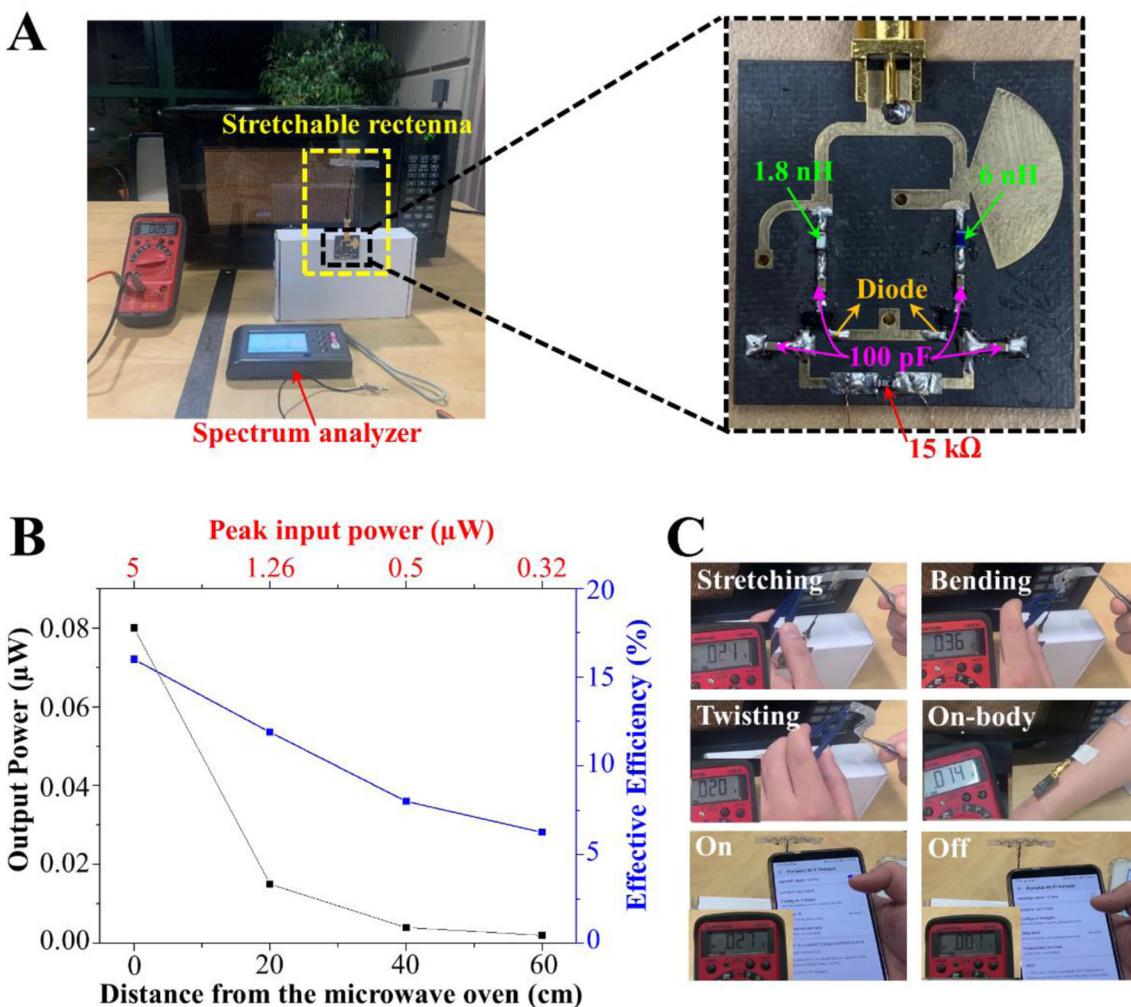
Figure 4. Energy harvesting performance of the stretchable wideband rectenna.
