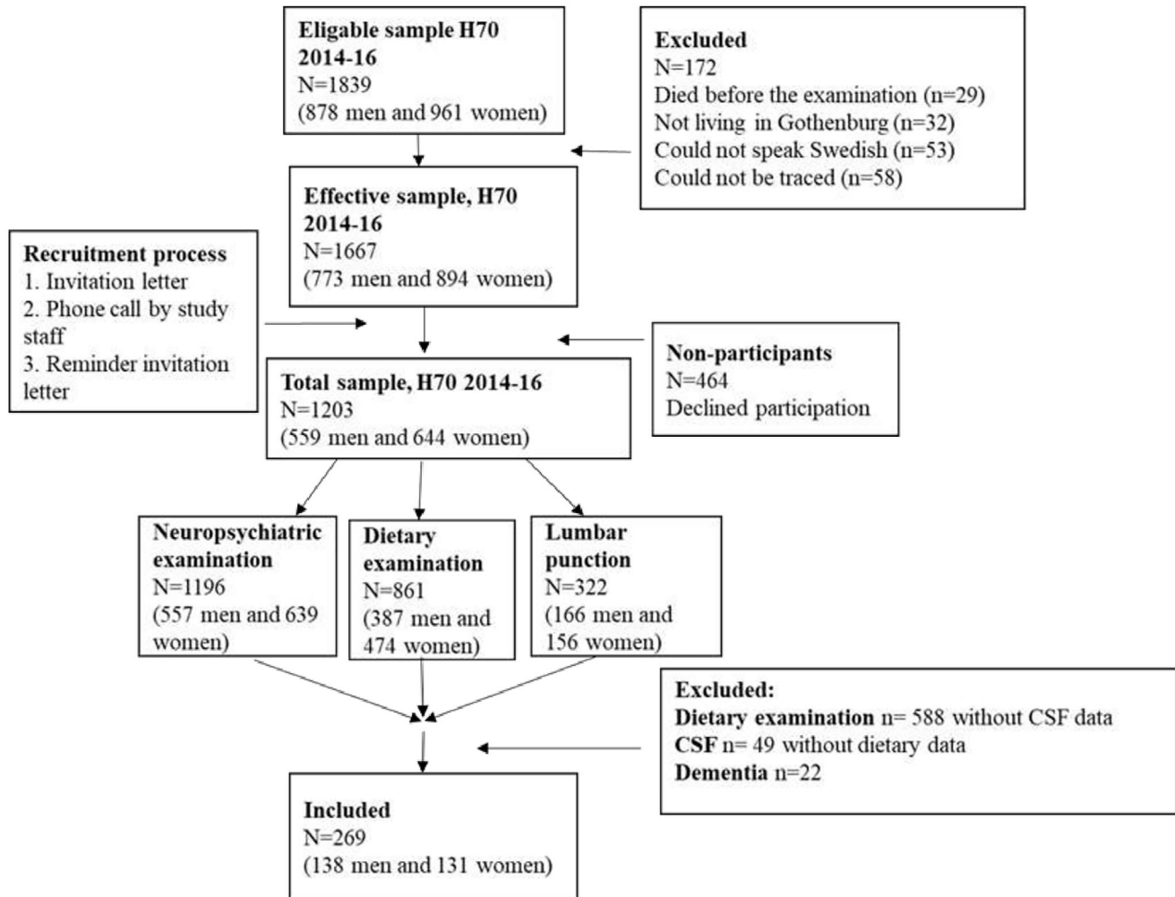
FIGURE 1 Sample flowchart
