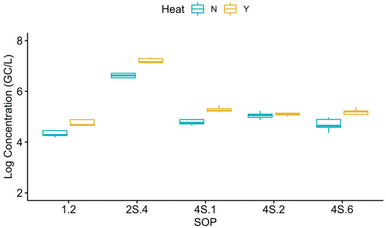
Fig. 7. Impact of heat pasteurization on the log-transformed SARS-CoV-2 (N1 target) concentrations (corrected for recovery efficiency) at Plant 1. Five sample replicates for each SOP, with and without heat pasteurization, were performed.
