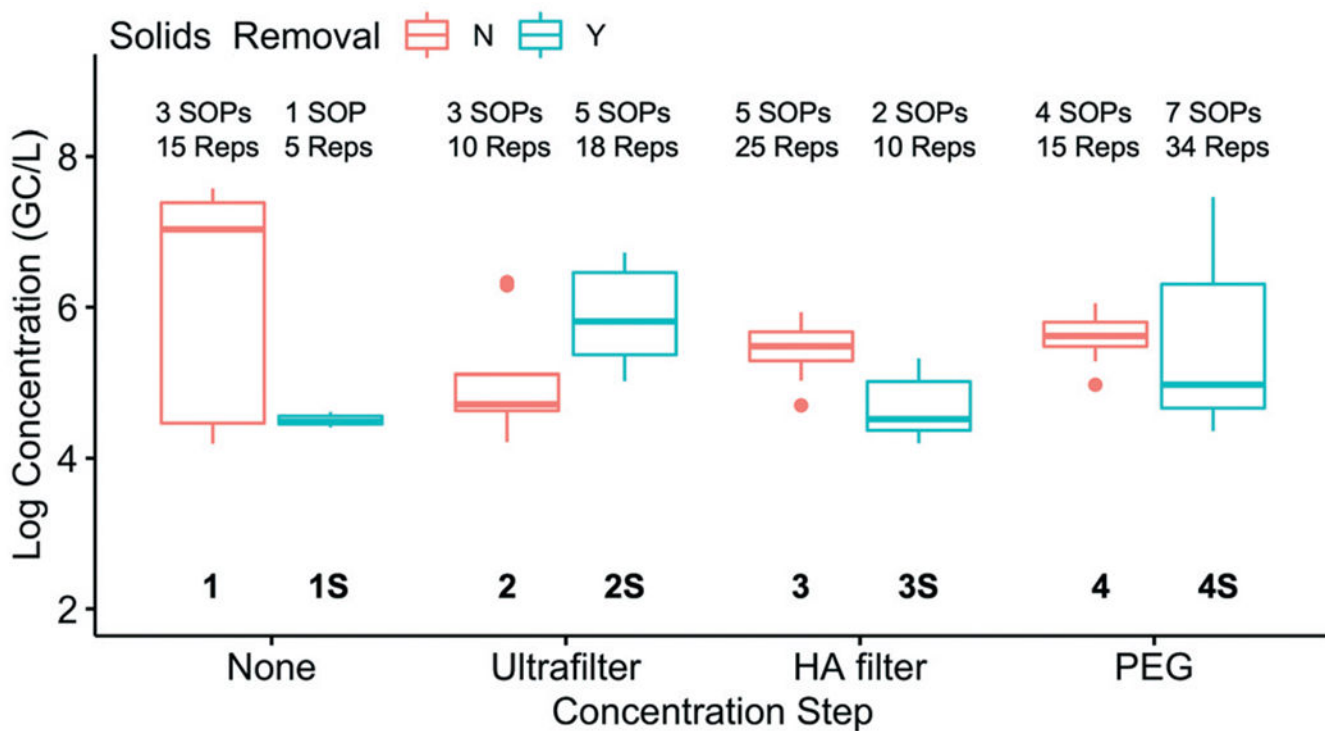
Fig. 3. Comparison of the log-transformed SARS-CoV-2 (N1) concentrations at Plant 1 measured by each of the eight method groups (grouped by concentration step and solids removal). The number of SOPs and total sample replicates included in each method group are shown at the top of the box plot.
