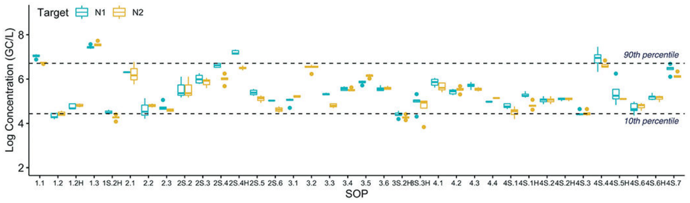
Fig. 1. Recovery-corrected SARS-CoV-2 concentrations (N1 and N2 targets) at Plant 1 measured by each SOP. NDs and data excluded based on the quality control criteria are not plotted. The dashed lines show 10th and 90th percentiles across all N1 and N2 results.
