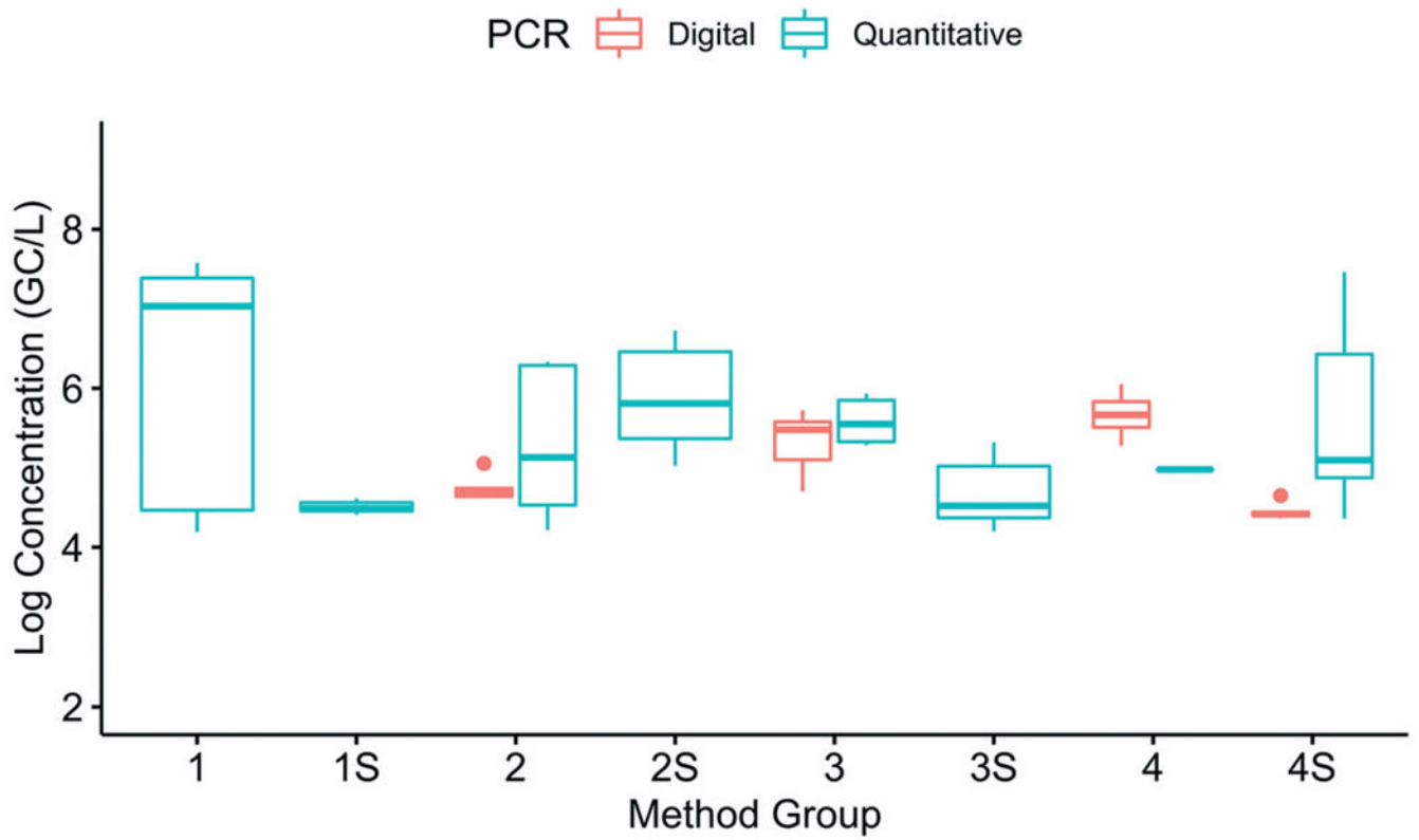
Fig. 8. Impact of the PCR platform (digital or quantitative) on the log-transformed SARS-CoV-2 (N1 target) concentrations (corrected for recovery efficiency) at Plant 1. The data are from 22 SOPs (93 replicates) that used quantitative PCR and 8 SOPs (39 replicates) that used digital PCR.
