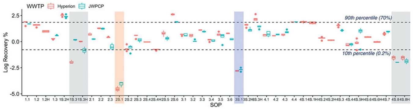
Fig. 2. Log-transformed OC43 recovery efficiency at Plant 1 (Hyperion) and Plant 2 (JWPCP), measured by each SOP. The SARS-CoV-2 results from the SOPs highlighted are not represented in Fig. 1 due to the fact that the results were all non-detect (gray), the recovery was below the quality control cut-off of 0.01% (blue), or both (orange).
