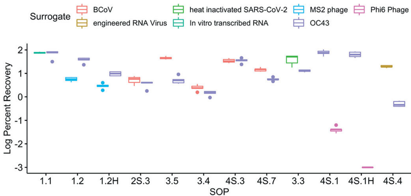
Fig. 9. Impact of the surrogate used for the matrix spike on the log-transformed recovery efficiency at Plant 1. Five sample replicates for each SOP were processed and analyzed for both OC43 and the second matrix spike surrogate.
