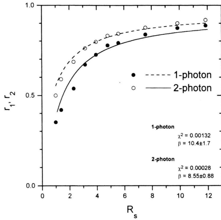
Fig. 6. Dependence of r_1 and r_2 on the degree of stretching, R_s , for HOE in PVA films for OPE (●) and TPE (○) excitation.
