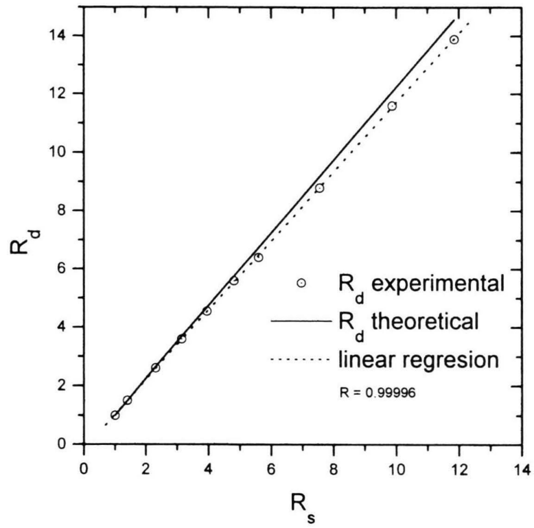
Fig. 5. Theoretical dependence of the dichroic ratio R_d on the stretch ratio R_s for \varphi = 0^\circ ((9) and (4) in [9]); \odot - experimental points.
