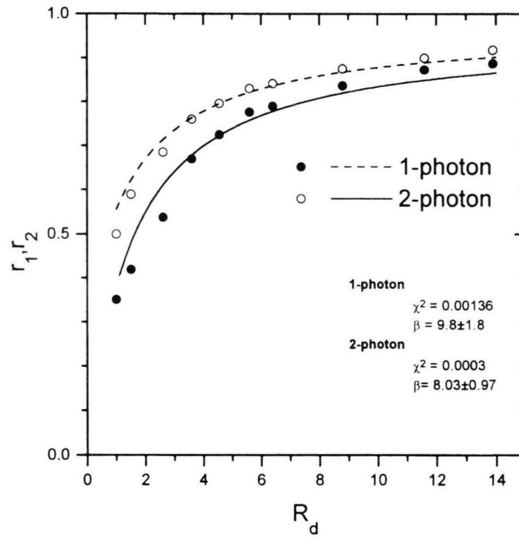
Fig. 7. Dependence of r_1 and r_2 on the dichroic ratio R_d = \frac{A_{\parallel}}{A_{\perp}} for HOE in PVA films for OPE (●) and TPE (○) excitation.
