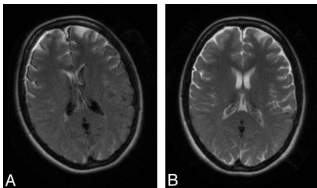
Fig 2. Healthy volunteer. Transverse standard single-shot, fast spin-echo, fluid-attenuated inversion recovery (SS-FSE-FLAIR) images with moderate rotation (A) and moderate nodding (B). The high signal intensity in the subarachnoid space and ventricular system is more extensive in panel B.
