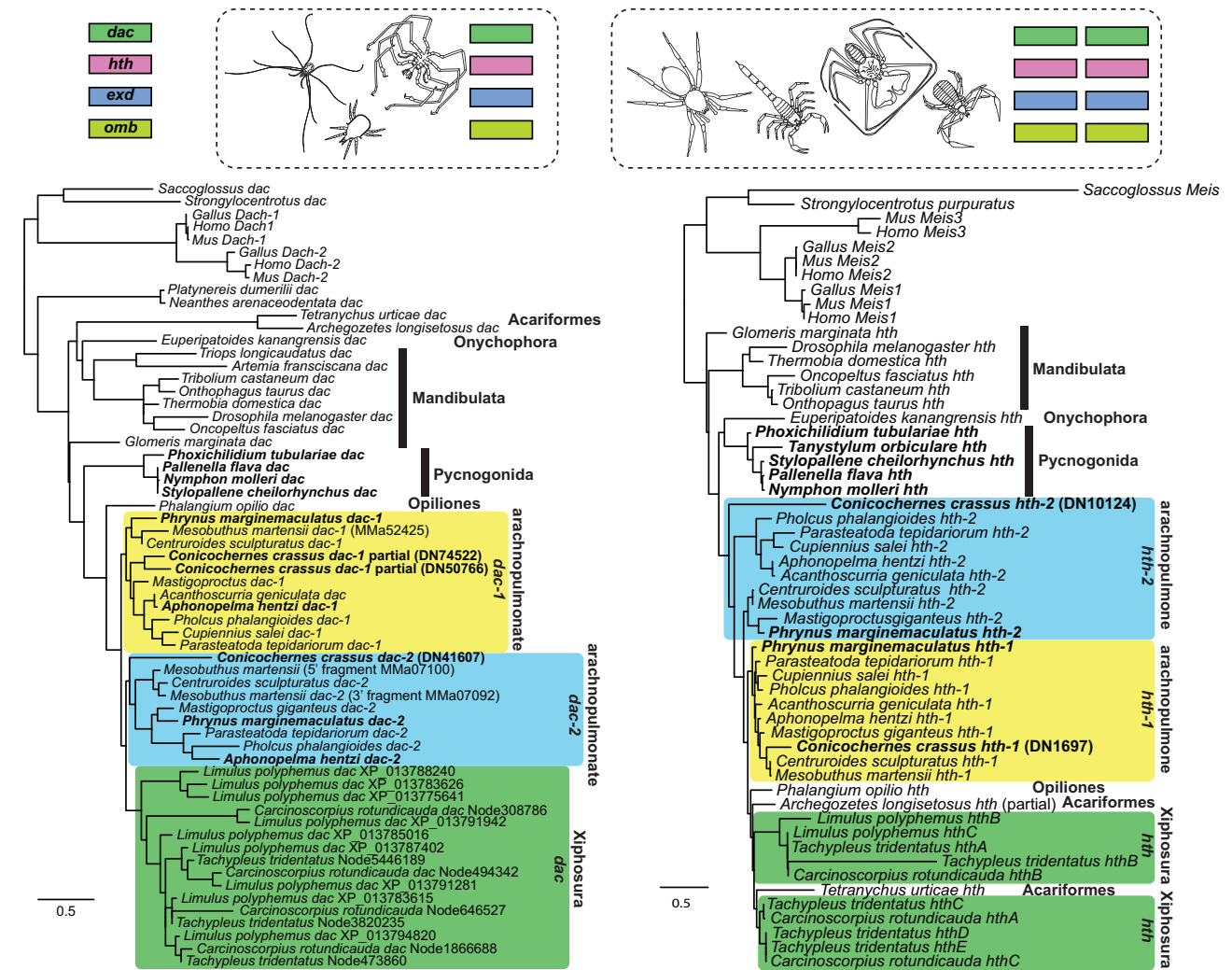
Fig. 7. Pseudoscorpions possess two copies of four developmental patterning genes known to exhibit paralogs with arachnoplumonate-specific spatiotemporal expression domains. Above: Single copy orthologs of dac , hth , exd , and omb were recovered from genomic resources for sea spiders, harvestmen, and Acariformes, whereas two copies of each gene were recovered for scorpions, tetrapulmonates, and pseudoscorpions. Below left: Maximum likelihood gene tree topology of the medial leg gap gene dac . Below right: Maximum likelihood gene tree topology of the proximal leg gap gene hth . Note the clustering of pseudoscorpion copies within arachnoplumonate clusters. dac-1 of C. crassus was recovered as two non-overlapping fragments.
