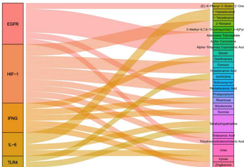
Figure 3 BXXX and its major components target and regulate key factors in the PD-L1 pathway.
