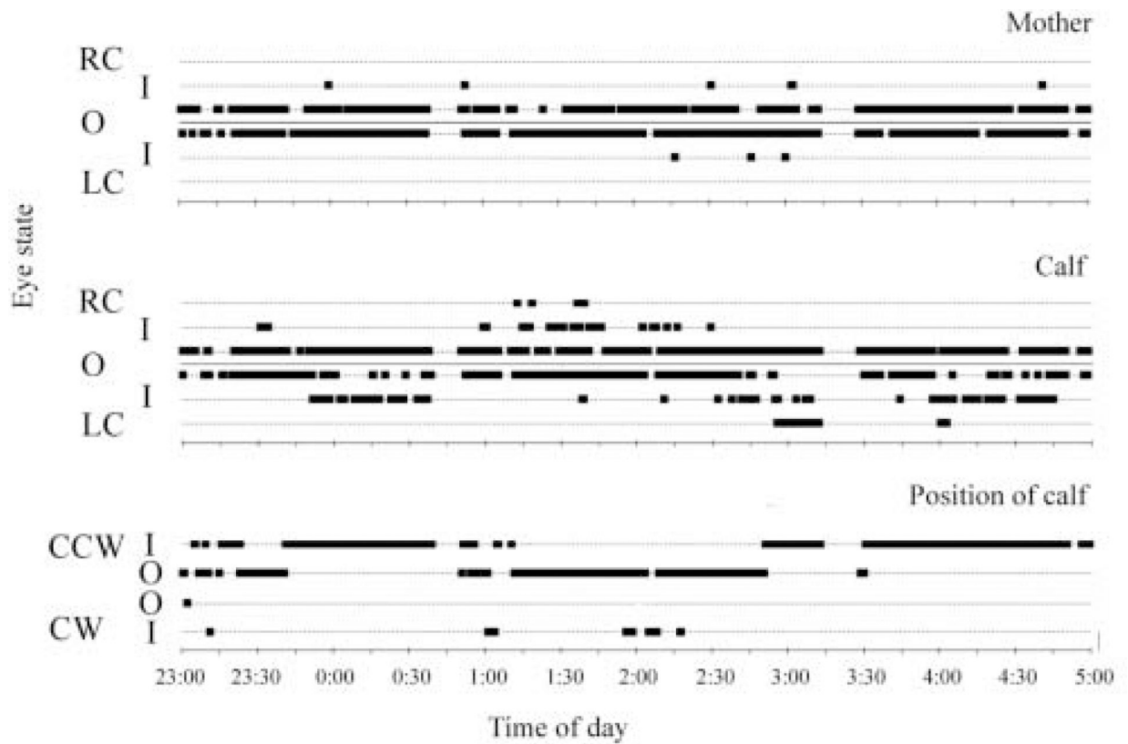
Figure 3. Simultaneous recording of eye state in a bottlenose dolphin mother and her calf (pair 2) during slow circular swimming. The state of each eye (R -right, L -left) is marked as open (O), closed (C) or intermediate (I). The position of the calf relative to its mother is shown as inner (I) or outer (O). The direction of swimming in the dolphin pair is marked as counterclockwise (CCW) or clockwise (CW). Interruptions in the record of eye state and calf position (at 0:45 and 3:15) represented gross periods of activity during which time dolphin eyes could not be continuously monitored. However, when visible, both eyes were open at these times.
