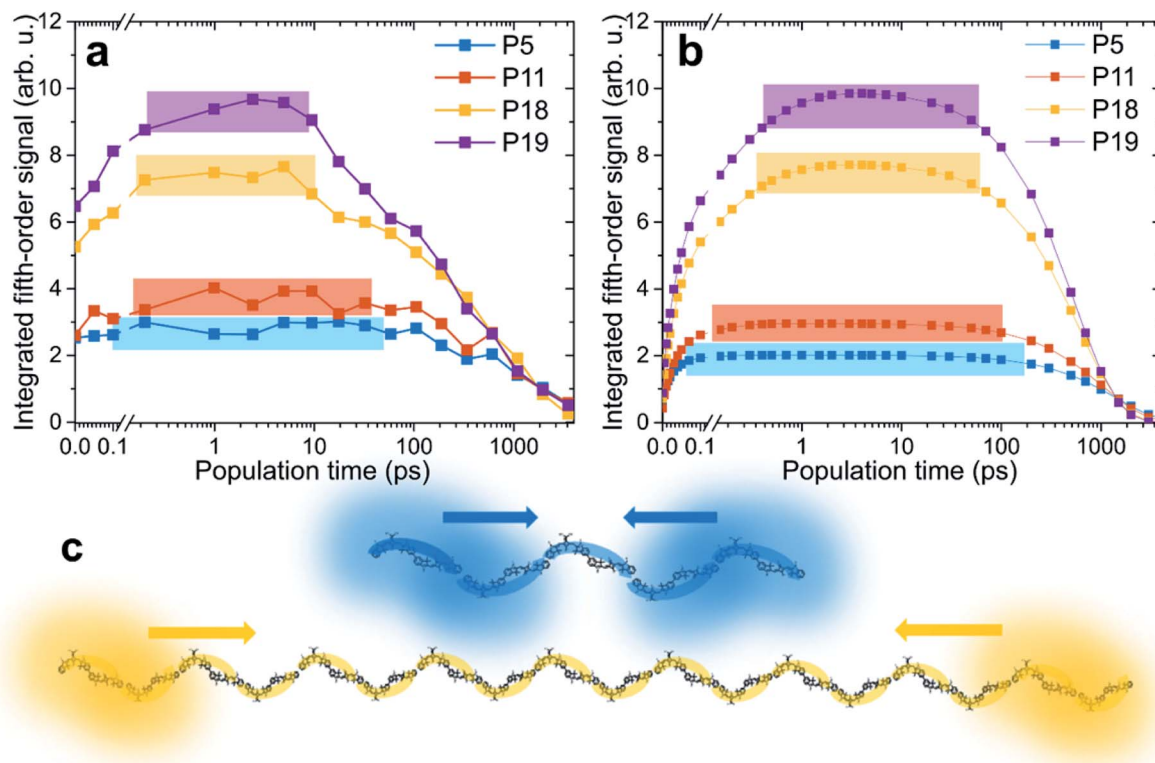
Fig. 3 Time-dependent results from EEI2D spectroscopy. (a) Measured and (b) calculated evolution of integrated fifth-order signals as a function of population time. The colors indicate the varying length of the polymers. The rectangles determine the regions within which the signal exceeds 90% of its maximum (see text for details). The data were normalized on the decaying tail. (c) Exemplary illustration of excitons in P5 and P18 polymers. The excitons are delocalized over a significantly larger fraction of the polymer in P5 than in P18 and therefore interact sooner after photoexcitation.
