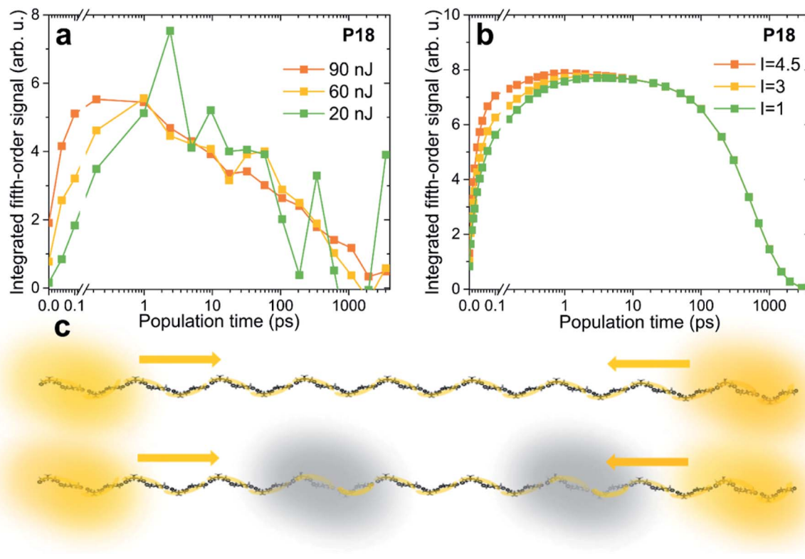
Fig. 5 Power dependence of the integrated EEI2D signal. Comparison of (a) measured and (b) calculated traces for excitation pulse energies of 20 nJ (green), 60 nJ (yellow), and 90 nJ (orange). (c) Larger excitation power leads to faster signal rise due to prompt annihilation by a population of excitons that are not directly probed, depicted in this cartoon in gray.
