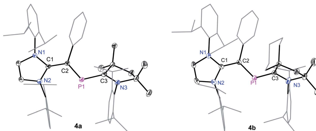
Fig. 4 Solid-state molecular structures of radical cation 4a and 4b . Hydrogen atoms, solvent molecules in 4b , and the counter anions GaCl_4^- have been omitted for clarity. Selected bond lengths and bond angles are given in Table 1.
