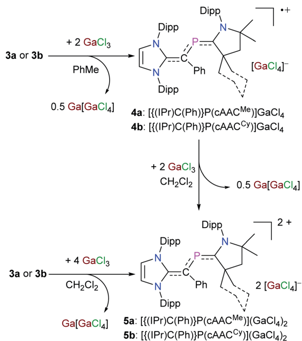
Scheme 2 Sequential one-electron oxidation of 2-phospha-1,3-butadienes 3a and 3b with GaCl_3 to the corresponding radical cations 4a and 4b and dications 5a and 5b .
