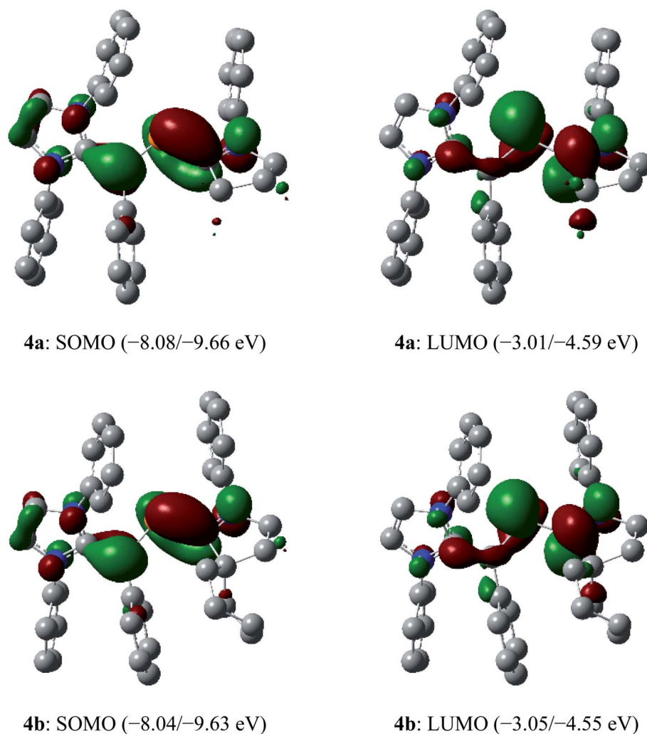
Fig. 6 Selected molecular orbitals (isovalue 0.04) of the radical cations 4a and 4b ( \alpha/\beta spin orbital energy) calculated at the M06-2X/def2-TZVPP//def2-SVP level of theory. Hydrogen atoms, methyl groups as well as iso-propyl groups were omitted for clarity.
