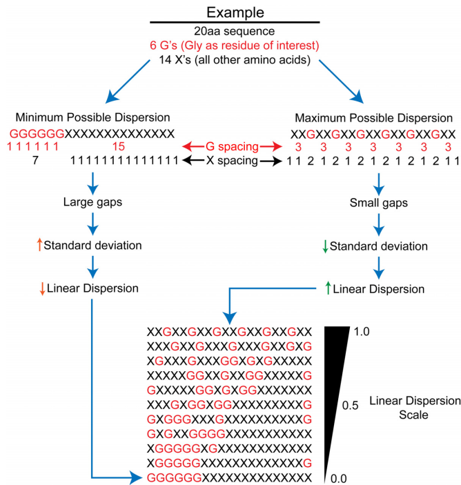
Figure 1. Depiction of linear dispersion parameter. Linear dispersion is calculated from the normalized standard deviation in the combined spacing values for all residues of interest and all other residues. Large gaps lead to large standard deviations, resulting in low linear dispersion values. Conversely, small gaps with uniform spacing leads to small standard deviations and high linear dispersion values. The linear dispersion scale ranges from 0.0 to 1.0, with high linear dispersion values indicating well-mixed sequences.
