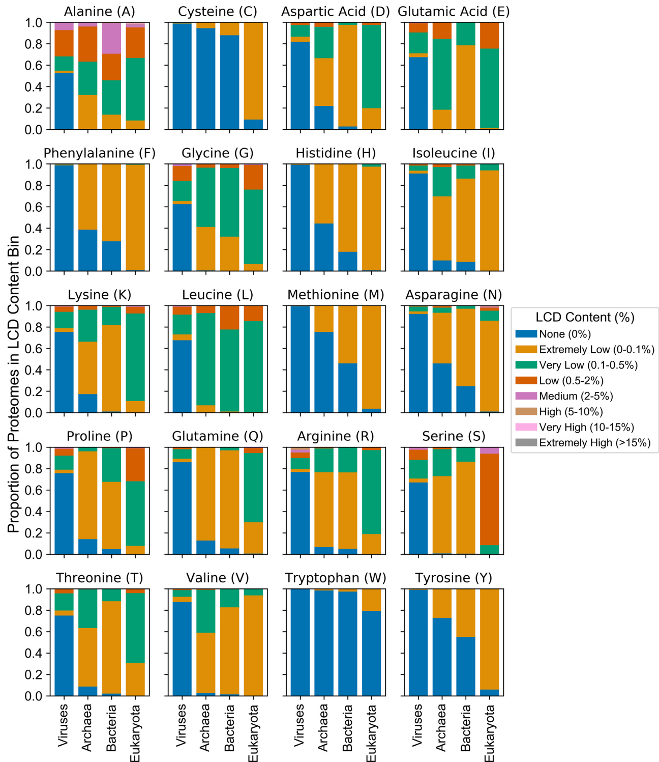
Figure 4. Cross-domain comparison of LCD content across all proteomes for each LCD class. LCDs were identified using LCD-Composer with default parameters for all proteomes available from UniProt. For each LCD class, the percentage of each proteome classified as LCD was defined as the percentage of amino acids lying within LCD regions out of the total proteome size (in number of amino acids). Within each domain of life, organisms were then sorted into one of seven categorical bins based on the percentage of the proteome classified as LCD for each LCD class [none (0%), extremely low (0–0.1%), very low (0.1–0.5%), low (0.5–2%), medium (2–5%), high (5–10%), very high (10–15%), or extremely high (>15%)]. The proportion of total proteomes for each domain of life was then calculated for each bin and plotted as a stacked bar chart. For all organisms, the ‘additional’ file containing sequences of known protein isoforms (when available) was combined with the corresponding organism’s main proteome prior to analyses.
