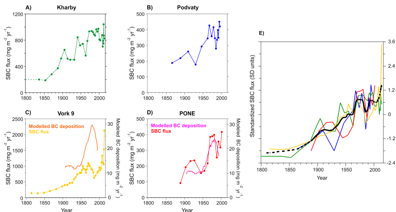
Figure 2. Sedimentary and standardized SBC fluxes observed in the Russian study lakes from 1800 to 2014 and modeled BC deposition between 1900 and 1999. (A–D) SBC fluxes ( \text{mg m}^{-2} \text{yr}^{-1} ) in the sediment records. Note different y-axes between the lakes. Observations in Kharby and Vork 9 connected by dashed lines are from sediment sequences that have not been dated, and their age is estimated based on the sedimentation rate of the last dated sample. (C,D) Additionally, the modeled BC deposition to Vork 9 and PONE is shown on their own y-axes ( \text{mg m}^{-2} \text{yr}^{-1} ) as 10-year running averages from 1900 to 1999. (E) Stacked SBC fluxes at Kharby, Podvaty, Vork 9, and PONE expressed as standard deviations from the mean. The black curve indicates a LOESS smoother (span 0.15) fitted to all records shown as dashed lines for time periods for which data are available only for some of the lakes.
