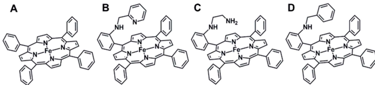
Fig. 2 Molecular structures of iron–porphyrin complexes used in this study: (A) Fe III TPP, (B) Fe III L2, (C) Fe III L3 and (D) Fe III MPh.
