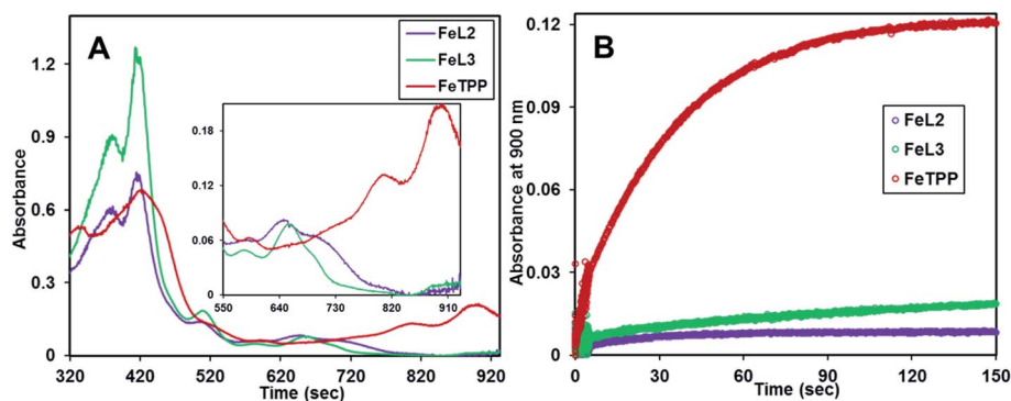
Fig. 5 Rapid-scan electronic absorption spectra of the reaction of iron porphyrin complexes (50 \mu\text{M} ) with 8 equivalent of meta -chloroperbenzoic acid ( m -CPBA, 200 \mu\text{M} ) in dichloromethane followed at -30^\circ\text{C} . (A) Selected overlay spectra representing the intermediate species formed after 50 s of the reaction, (B) overlay of the time traces at the 900 nm band with the formation of isoporphyrin species ( \lambda_{\text{max}} = 900 \text{ nm} ) for these three complexes (Fe III TPP(Br) (red line), Fe III L2(Br) (violet line) and Fe III L3(Br) (green line)).
