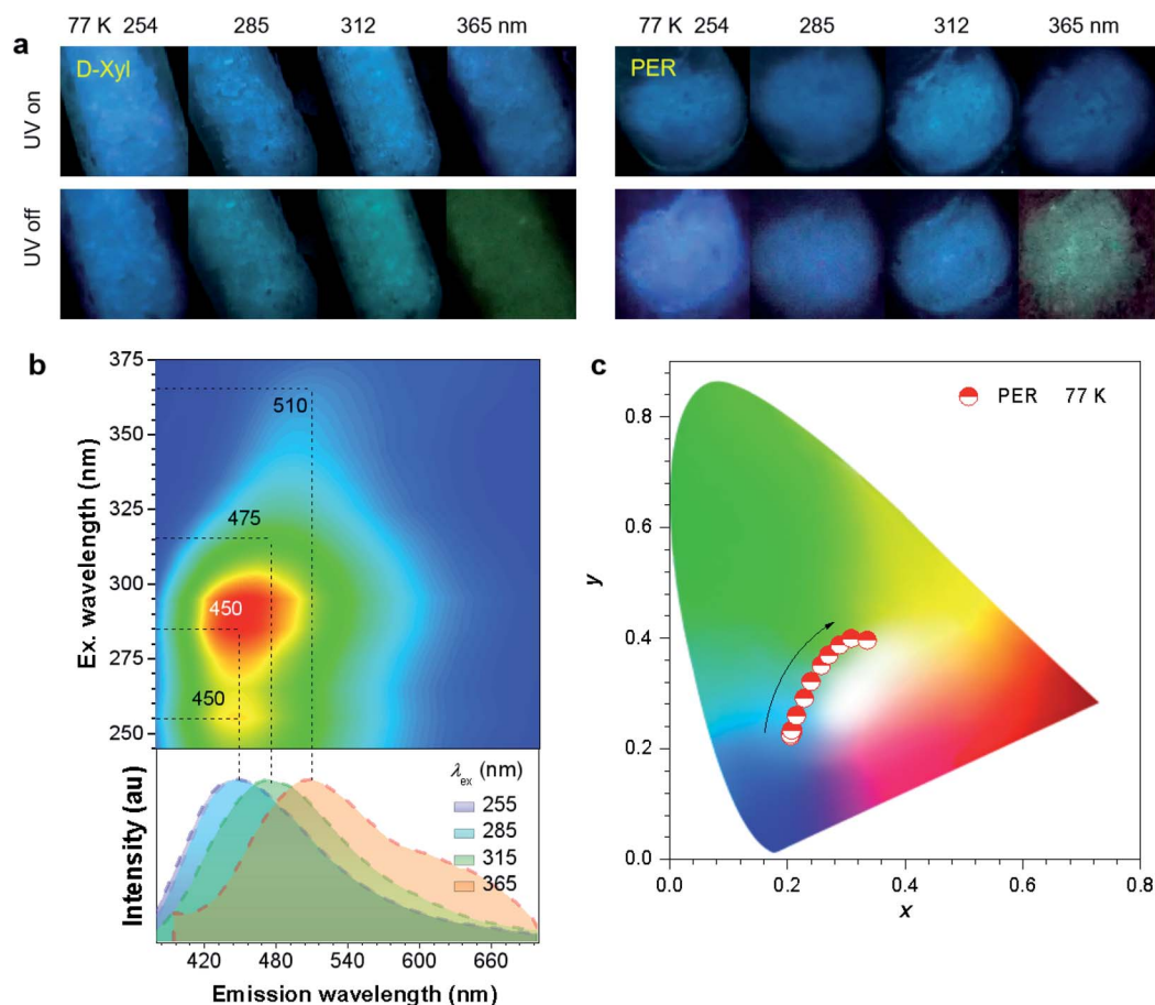
Fig. 4 (a) Photographs of D -Xyl and PER crystals taken at 77 K under varying UV light wavelengths or after stopping the irradiation. (b) Excitation–phosphorescence mapping and the phosphorescence spectra with different excitations ( t_d = 0.1 ms) of PER crystals at 77 K. (c) Trajectory of phosphorescence colors of PER crystals at 77 K, recorded by the change in the \lambda_{ex} from 245 to 375 nm, in the CIE coordinate diagram.
