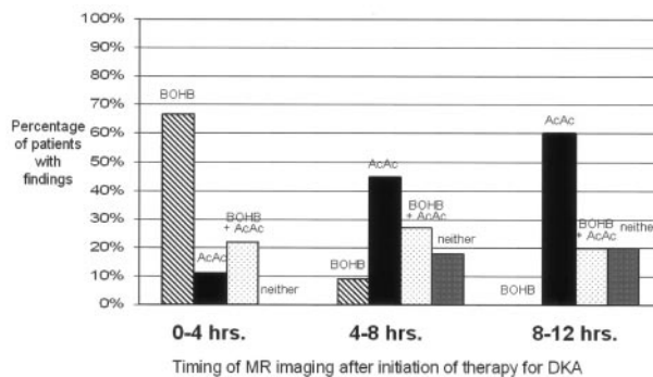
FIG 2. Patients with \beta OHb, AcAc, both, or neither on initial imaging during DKA therapy.
