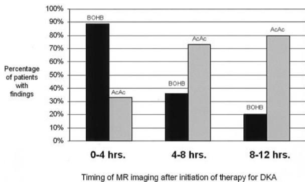
FIG 4. Patients with \beta OHB and/or AcAc on initial imaging by the timing of the study after the start of therapy.
