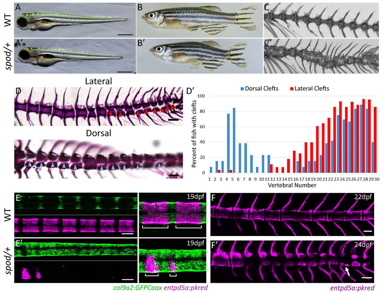
Figure 1. The spodo mutant impairs axial patterning and leads to the formation of hemicentra. A) spodo mutant zebrafish are viable. 4dpf larval morphology of wild-type and cmn spod heterozygous larvae. Mutants show normal patterning of larval structures, however, are shorter in length. B) cmn spod/+ mutants are viable and exhibit short stature as adults. Tomographic reconstruction of vertebrae of wild-type C) and spodo heterozygous C') adult fish showing formation of hemicentra and periodic diplospondyly (arrow). Homozygous fish show an increase in phenotype, (Figure S1). D) Lateral and dorsal views of cmn spod/+ alizarin red stained skeletal preps. Hemicentra are present along the body axis. Arrows indicate vertebral clefts. D') The frequency of vertebral clefts along the body axis was quantified. Dorsal clefts were found bimodally in the rostral and caudal regions of the vertebral column while lateral clefts were most prominent in the caudal region and associated with non-rib-bearing vertebrae. E) Early specification of notochordal patterning is disrupted in spodo mutants. In wild-type fish, col9a2:GFPCaax expression is restricted to the prospective intervertebral discs (IVD) while entpd5a expression is activated in the mineralizing domains (future chordacentra) of the notochord sheath. bottom) E') Specification of the IVD and mineralizing domains is absent in spodo mutants, while the expression domain of col9a2 is expanded. Overlay of entpd5a and col9a2 transgenes
