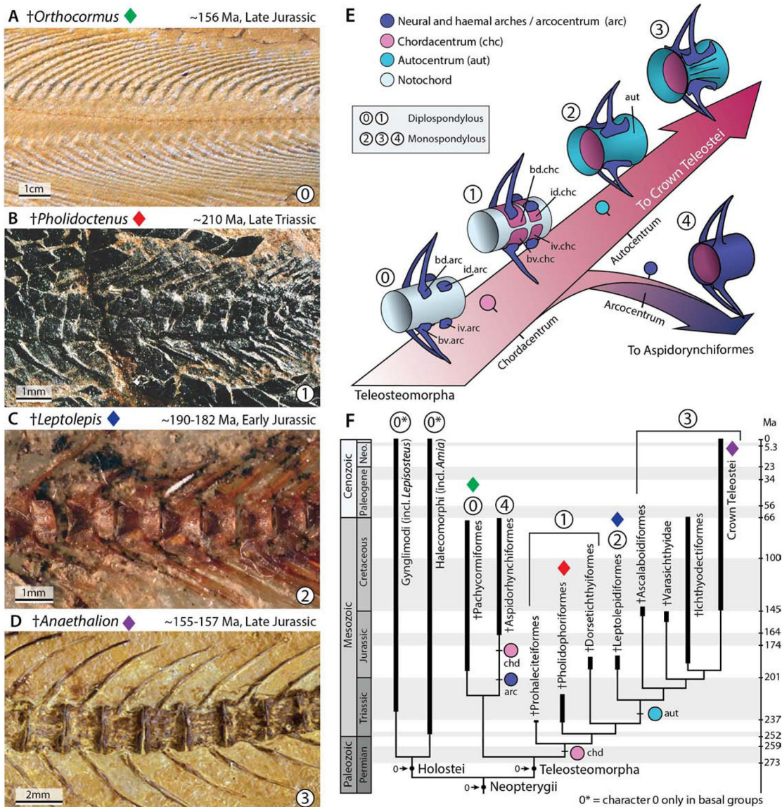
Figure 2. Patterning of the spine and the evolution of the teleost vertebral centrum. Reconstructing the changes in spine patterning and morphology during the evolution of teleosts. A) The earliest members of stem teleosts lacked a vertebral centrum, and instead retained a functional notochord supporting the arches and spines. This is illustrated by the stem pachycormiform † Orthocormus roeperi ; see also E) state “0” . B) † Pholidoctenus serianus illustrates a more derived condition present among some pholidophoriforms, with diplospondylous vertebral centra formed by hemi-chordacentra; E) state “1” . C) † Leptolepis coryphenoides illustrates a major transformation within the spine of stem teleosts, characterized by the appearance of a thin hourglass-shaped autocentrum surrounding a ring-like chordacentrum; E) state “2” . D) Subsequently, the autocentrum incorporated a thickened lateral wall, and a series of ornaments, such as crest, grooves and pits, as illustrated by the oldest fossil member of the teleost crown group † Anaethalion sp., a condition retained in, and defining all living teleosts; E) state “3” . E) Reconstructed scenario of the evolution of
