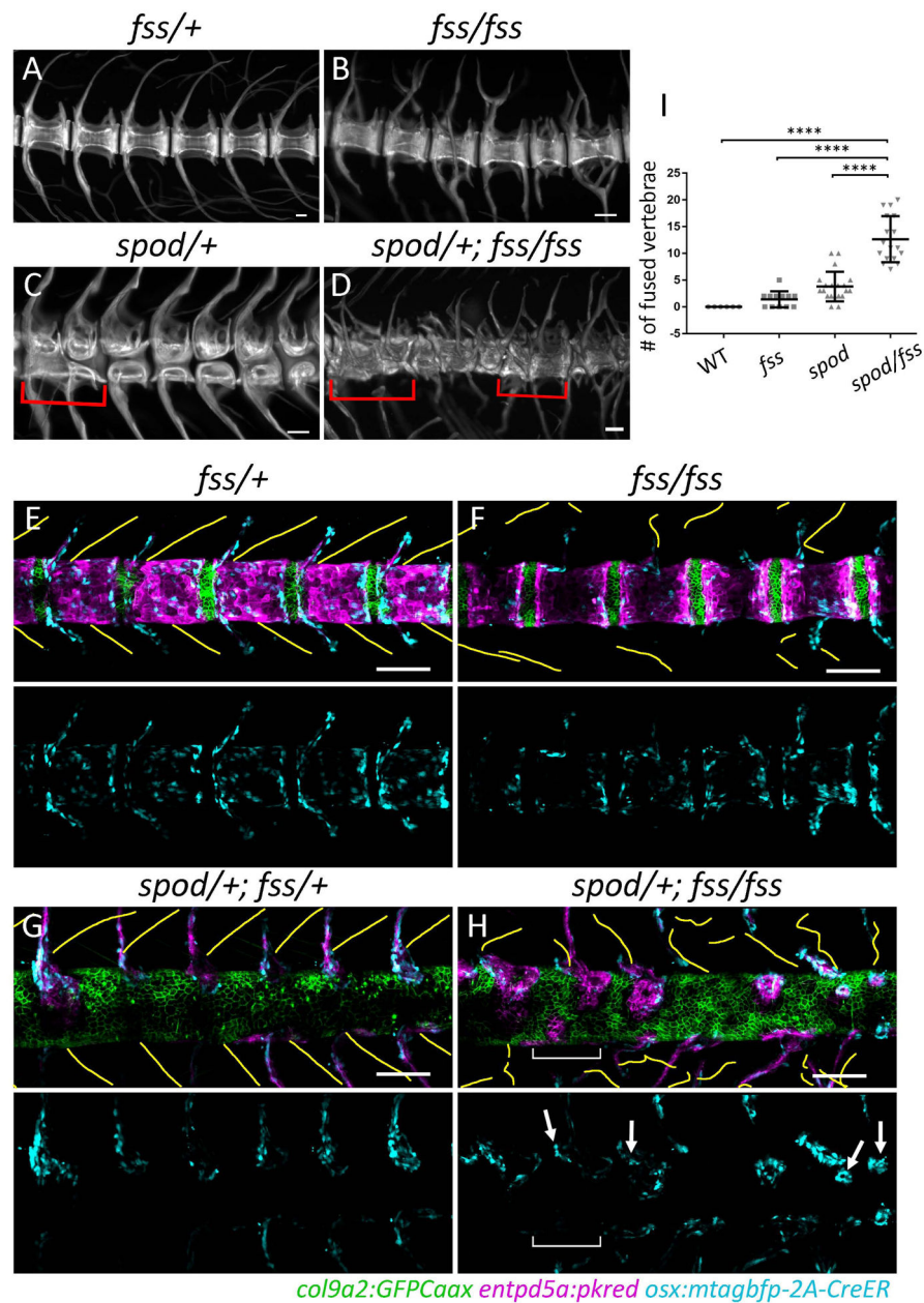
Figure 5. Sensitization of cmn spod mutants to tetrapod segmentation programs. A-D) Alizarin red stained skeletal preparations at 6wpf. A) Wild-type skeletal preps demonstrate meristically patterned autocentra and arches. B) tbx6 fss/fss mutants display irregular arch morphology and patterning while centra remain regularly segmented. C) cmn spod/+ mutants have the opposite phenotype wherein arch patterning is normal and the centra contain large vertebral clefts. D) Double mutants in which both notochord and somite segmentation have been disrupted are not simply a combination of the two aforementioned phenotypes. In contrast, double mutants form highly irregular vertebral structures with very little discernable patterning. Red brackets indicate vertebral fusion events. E) The number of fused vertebrae in each condition was quantified along the body axis using alizarin red
