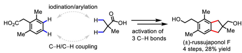
Scheme 1. C–H Activation/C–C Bond-Forming Reactions
