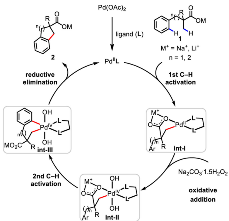
Scheme 3. Proposed Mechanism for Cyclative C(sp 3 )-H/C(sp 2 )-H Coupling Reaction
