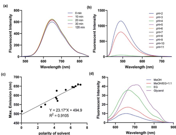
Fig. 2 (a) The fluorescent spectra changes of ICTAD-1 ( 10\ \mu\text{M} ) in DMF under the irradiation of daylight lamp for 120 min; (b) the fluorescent spectra of ICTAD-1 ( 10\ \mu\text{M} ) in different pH aqueous solutions (1% DMF); (c) the linear relationship between the polarity of solvent and the maximum emission wavelength; (d) the fluorescence spectra of ICTAD-1 ( 10\ \mu\text{M} ) in solvents of different viscosity, EG: ethylene glycol.
