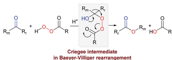
Scheme 1 Postulated mechanism of Baeyer–Villiger oxidation.
