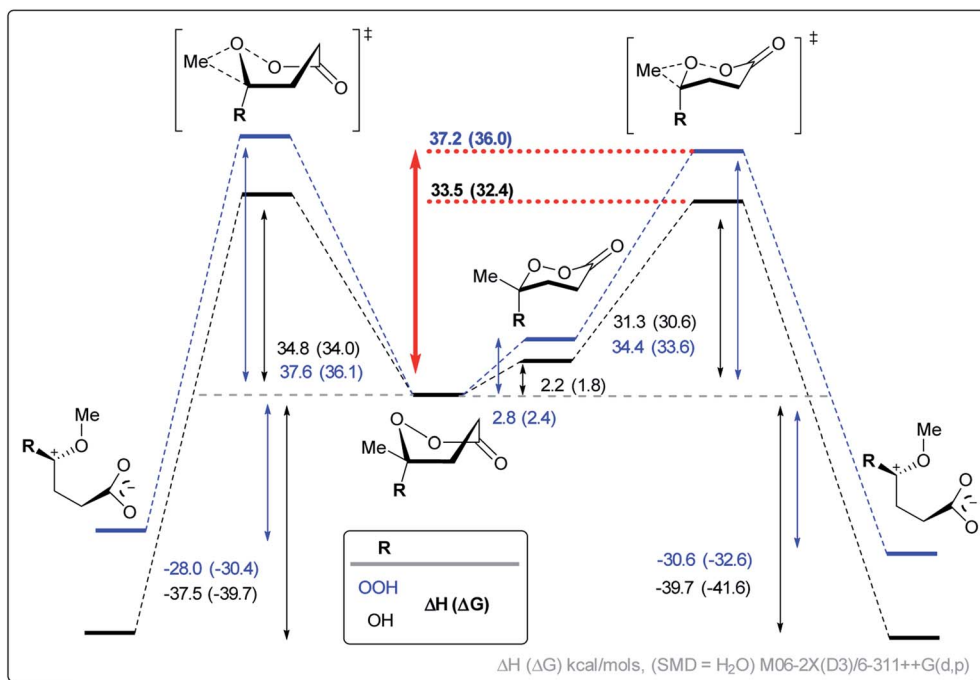
Scheme 11 Computational analysis of the BV 1,2-shift in cyclic CIs and their hydroperoxy analogs for the boat and chair conformations.
