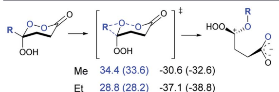
Scheme 9 Computational analysis of the BV 1,2-shift in cyclic Cls and their hydroperoxyl analogs for the chair conformations.
