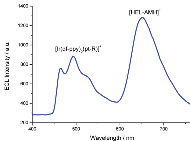
Fig. 3 ECL spectrum recorded in a PBS solution containing 10^{-4} \text{ M} [HEL-AMH] + and 10^{-3} \text{ M} [\text{Ir}(\text{df-ppy})_2(\text{pt-R})]^\dagger . Applied potential: 1.7 V vs. Ag/AgCl/KCl.
