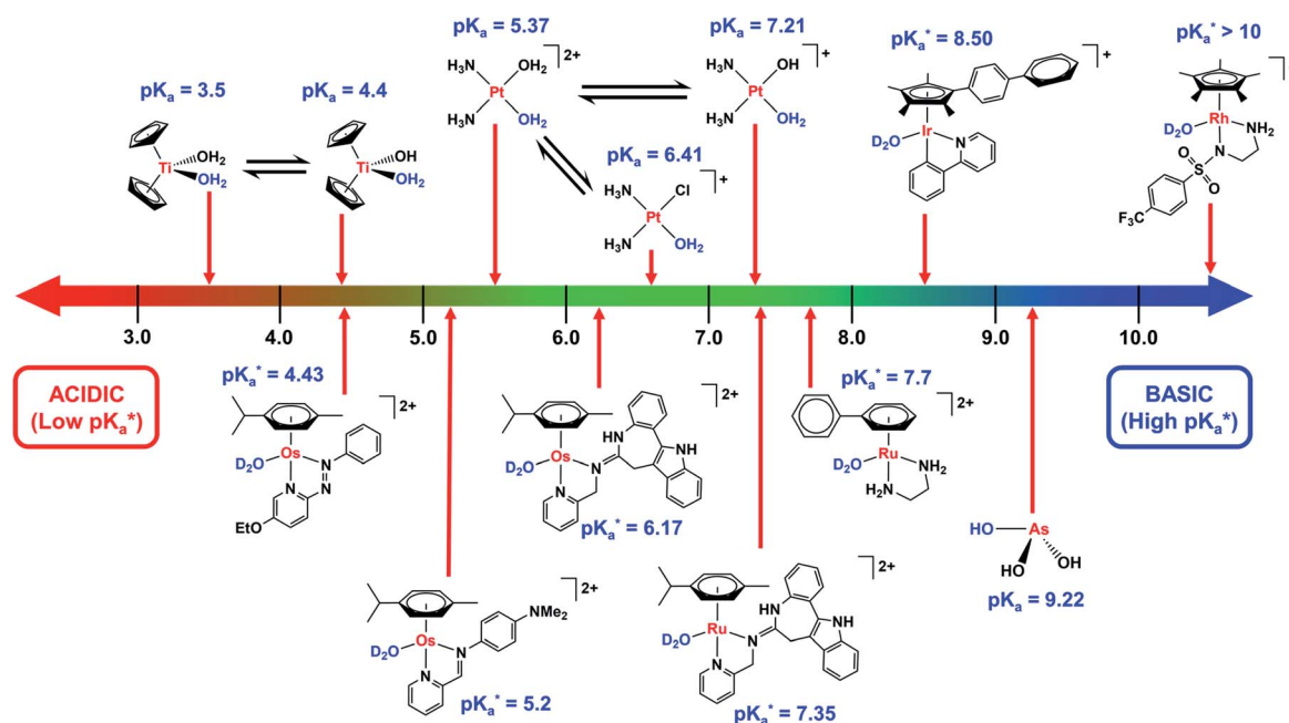
Fig. 3 Comparison of the \text{p}K_{\text{a}} values of aquated species of metal-based complexes. \text{p}K_{\text{a}}^* values refer to \text{M-OD}_2 complexes based on \text{pH}^* ( \text{pH} meter reading not corrected for the effect of deuterium on the electrode).
