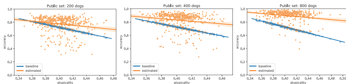
FIG. 5. Results of Figure 4 broken down by individual dogs. Here, each point represents a dog and we define atypicality as the proportion of uncommon variants that the dog has compared with the public database—for instance, if 51% or more of dogs in the public database have a G in a specific locus, but this dog has a T , then this would count toward the dog’s atypicality. In other words, dogs further to the right are less and less similar to average dogs present in the public dataset (measured by percentage of different variants). In contrast to the most-common-variant baseline, our method generalizes well even to dogs that are highly dissimilar to those in the public dataset. Larger public databases (right) provide more accurate population estimates of \hat{K} , leading to more accurate reconstructions overall.
