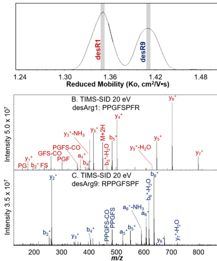
Figure 5. TIMS of a 1:1 mixture of desArg1 and desArg9 yielded baseline resolved distributions of the isobaric peptides (A). Reduced mobilities were calculated using Tune Mix as calibrant. Each distribution was selected (as indicated by gray slices), and the corresponding peptide was assigned based on the SID fragmentation spectra (B and C).
