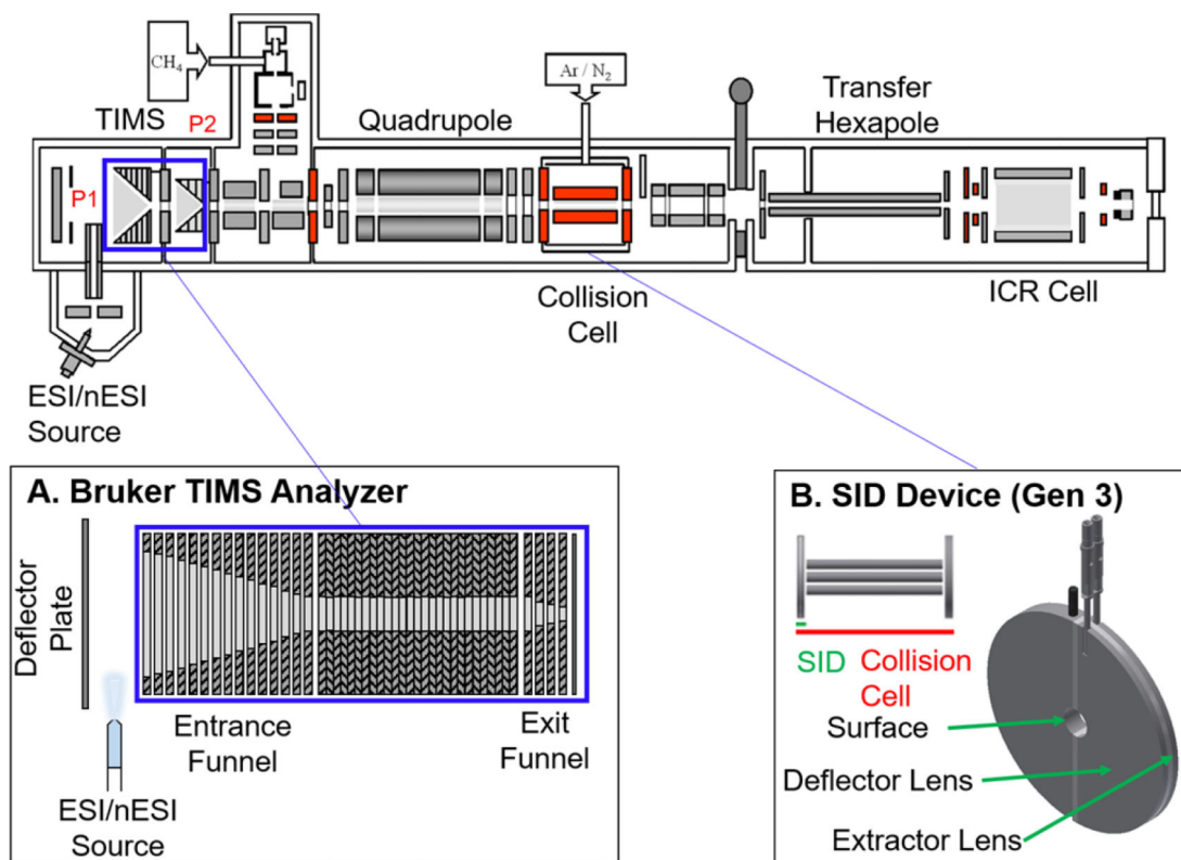
Figure 1. Instrument design and modifications, including a TMS analyzer 30 (A) and SID device 44 (B). The TMS analyzer replaced the entrance funnel (original entrance funnel region shown in blue box) and the SID device replaced the front-end cap of the commercial collision cell. The previously described SID device consists of three lenses: a semicircular surface onto which ions collide and two lenses with a non-conducting space in between: a deflector lens to push ions into the surface and an extractor lens element to extract and guide ions into the collision cell for accumulation prior to being pulsed into the ICR cell for detection. 44
