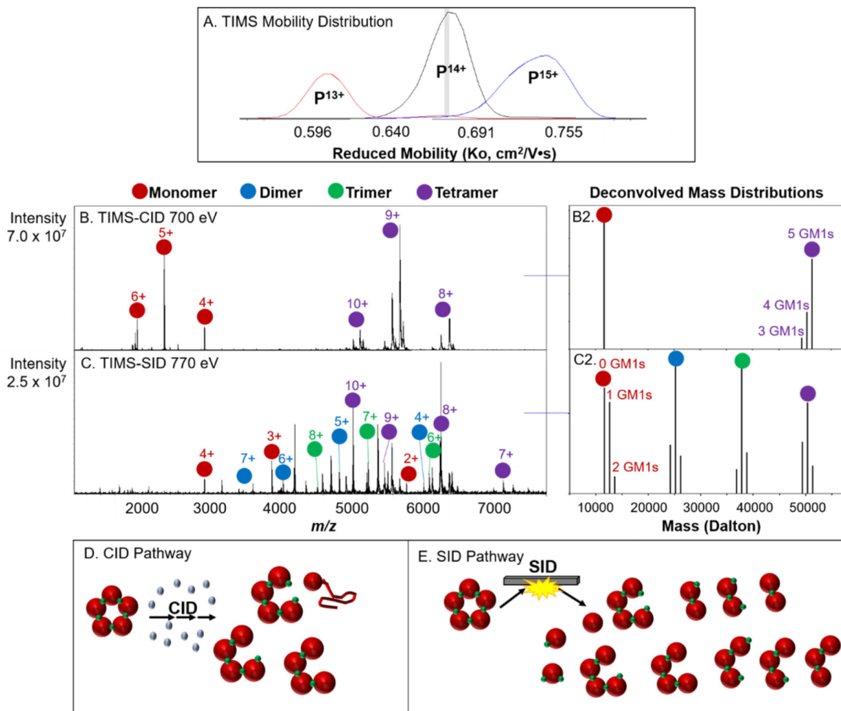
Figure 4. TIMS mobility distribution of CTB pentamer with GM1s ligand bound with mobility selection for CID and SID experiments highlighted with gray slice (A). Reduced mobilities were calculated using the protein/protein complex calibration. TMS-CID and TMS-SID of mobility-selected 14+ (B, C) with corresponding deconvolution to show variations of GM1s retention on subunits (B2, C2). CID and SID pathways of CTB with GM1s and the observed products (D, E).
