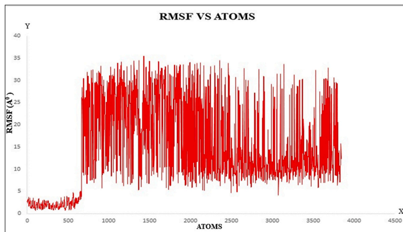
Fig. 6. Molecular Dynamics (MD) simulation of guide siRNA-argonaute complex A) Root Mean Square deviations (RMSD) plot, B) Root mean square Fluctuation (RMSF) plot.
