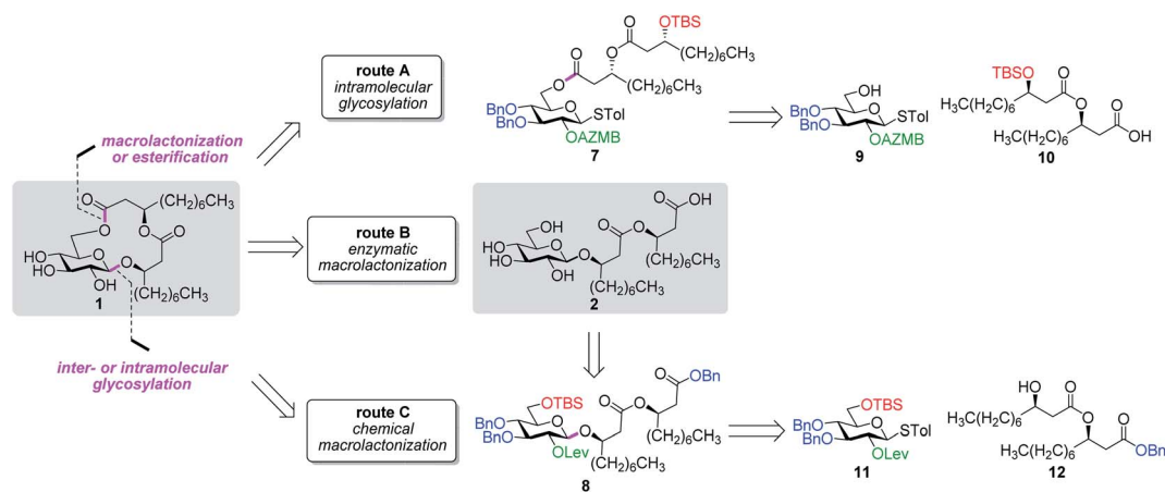
Fig. 2 Retrosynthetic disconnection strategy for the total synthesis of ananatoside A (1) and ananatoside B (2) according to three different pathways: chemical macrolactonization, enzymatic macrolactonization, and inter- or intramolecular glycosylation. AZMB: 2-azidomethylbenzoyl; Bn: benzyl; Lev: levulinoyl; STol: thiotolyl; TBS: tert -butyldimethylsilyl. Blue: permanent protecting groups (Bn); red: temporary protecting groups (TBS); green: esters used as temporary protecting groups enabling neighboring group participation (AZMB and Lev).
