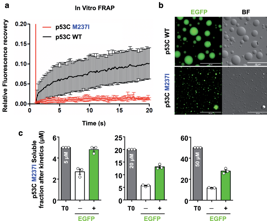
Fig. 6 Fluorescence recovery after photobleaching of p53 in vitro . (a) Line plot showing fluorescence recovery of wt and M237I p53C in the presence of 15% PEG. The data are shown as the mean \pm s.d. of n = 5 droplets. (b) Images showing the fluorescence and the bright-field (BF) channels of spherical droplets of wt and M237I p53C at 4 °C (time, 0 s; scale bars, 20 \mu\text{m} ). (c) Scatter plots representing the soluble fractions after the kinetic assay of M237I p53C in the absence (–) or in the presence (+) of the EGFP-tagged protein. T0 corresponds to the monomer concentration used before kinetic assays. The data are shown as the mean \pm s.e.m. of n = 3 independent experiments using the same protein batch.
