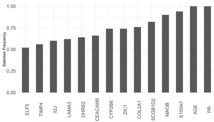
Figure 5: Selection frequencies for genes or phenotype variables that were selected at least 50% of the time with stability selection.
