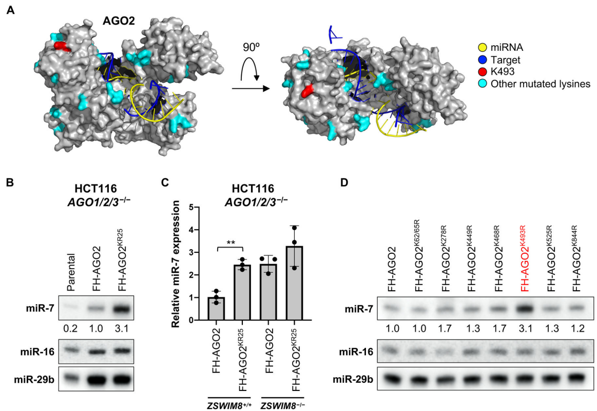
Fig. 4. Surface-exposed lysines in AGO2 are required for TDMD.
