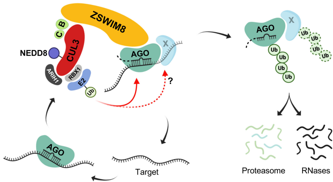
Fig. 7. Proposed model of ZSWIM8 ubiquitin ligase activity in TDMD.
