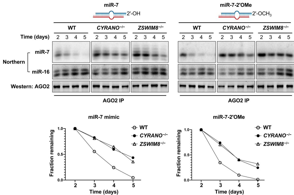
Fig. 5. miRNA tailing and trimming is not essential for TDMD.
