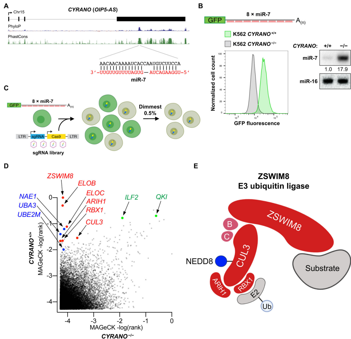
Fig. 1. A genome-wide CRISPR-Cas9 screen for TDMD factors reveals a cullin-RING E3 ubiquitin ligase.
