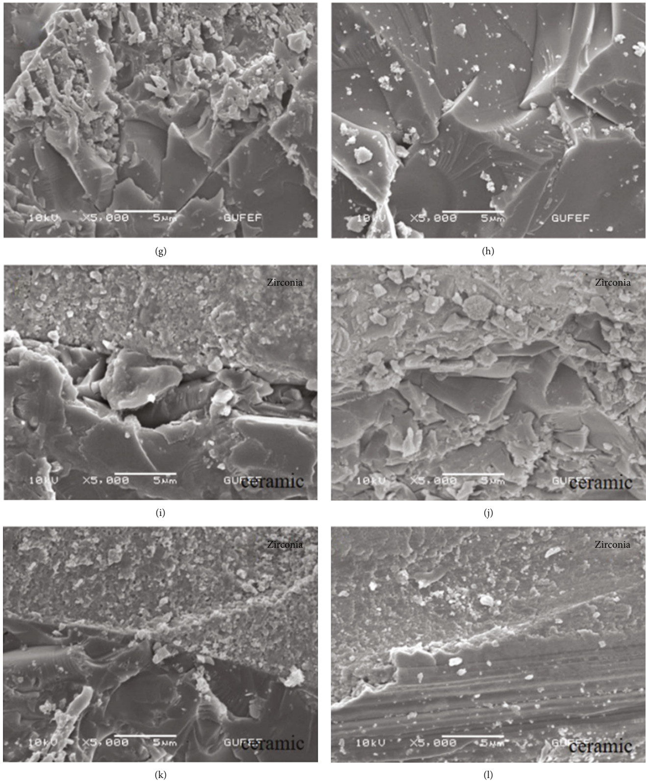
FIGURE 2: SEM images of the specimens after the surface treatments at a magnification of 5000x. (a) Zirconia-control (Group I-Subgroup I). (b) Zirconia-sandblasting (Group I-Subgroup II). (c) Zirconia-long-pulse laser (Group I-Subgroup III). (d) Zirconia-short-pulse laser (Group I-Subgroup IV). (e) Ceramic-control (Group II-Subgroup I). (f) Ceramic-sandblasting (Group II-Subgroup II). (g) Ceramic-long-pulse laser (Group II-Subgroup III). (h) Ceramic-short pulse laser (Group II-Subgroup IV). (i) Zirconia/ceramic-control (Group III-Subgroup I). (j) Zirconia/ceramic-sandblasting (Group III-Subgroup II). (k) Zirconia/ceramic-long-pulse laser (Group III-Subgroup III). (l) Zirconia/ceramic-short-pulse laser (Group III-Subgroup IV).
