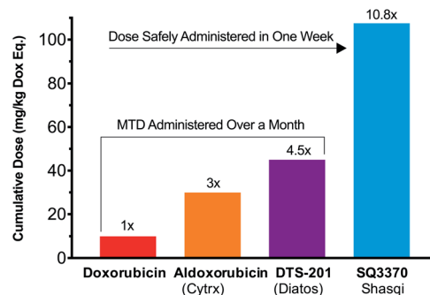
Fig. 3 Tolerability of SQ3370 as compared to Dox and clinically tested Dox-based treatments in rodents. (A) The cumulative MTD of SQ3370 in mice was determined to be 383 \text{ mg kg}^{-1} ( 76.6 \text{ mg per kg per day} \times 5 days), representing a 19.1-fold enhancement over the experimentally determined single-dose MTD of conventional Dox. (B) In rats, a cumulative dose of 107.5 \text{ mg kg}^{-1} ( 21.5 \text{ mg per kg per day} \times 5 days) was tolerated without overt toxicities, a 10.8-fold margin over the conventional Dox MTD administered as 4 weekly doses. 40 Previous Dox-based treatments have only been able to advance the MTD up to 60 \text{ mg kg}^{-1} in mice 40 and up to 45 \text{ mg kg}^{-1} , administered in two doses 22 days apart, in rats. 41 All doses here are represented in Dox eq.
