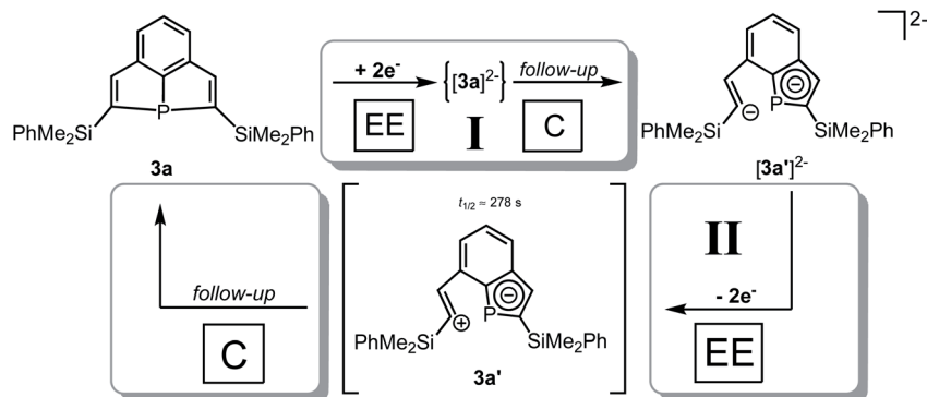
Scheme 2 Mechanism for the two-electron reduction I of tricyclic phosphine 3a to anion [\mathbf{3a}']^{2-} by an EEC mechanism and re-oxidation II mechanism via an EEC sequence involving a meta-stable intermediate 3a' .
