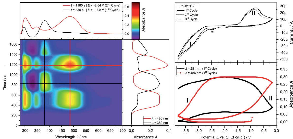
Fig. 2 Spectroelectrochemical CV measurement of the reduction I and reoxidation II ( v = -10 \text{ mV s}^{-1} ) of phosphine 3a (2.50 mM) in THF/0.1 M [ \text{Bu}_4\text{N} ][OTf] at a platinum grid electrode in a double compartment cuvette cell. Left contour plot: relative UV-vis spectral changes during 3 cycles of CV; middle vertical plot: time dependent UV-vis absorbance; top left: projected relative UV-vis spectra after reduction I (red line) and after reoxidation II (black line); top right: in situ CV, bottom right: absorption based CV.
