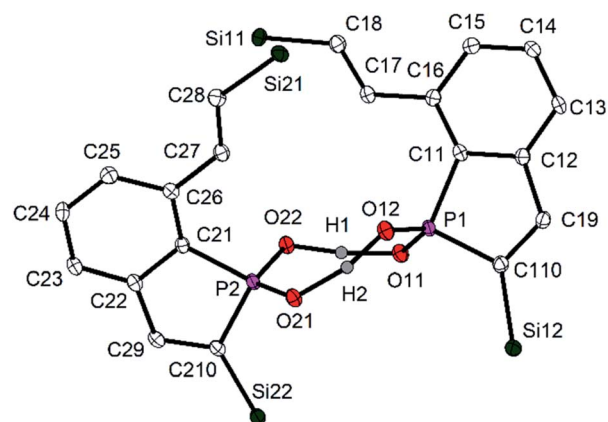
Fig. 9 Molecular structure and numbering scheme of 10 . Displacement ellipsoids are drawn at the 40% level; T = 100\text{ K} . H atoms with exception of H1 and H2 and the SiMe_2Ph groups except the central Si atoms are omitted. Important bond lengths (pm) and angles ( ^\circ ): P1–O11 153.7(2), P1–O12 151.6(2), P2–O21 153.4(2), P2–O22 151.8(2), P–C 179.6(av), O11–P1–O12 113.00(9), O21–P2–O22 112.85(9).
