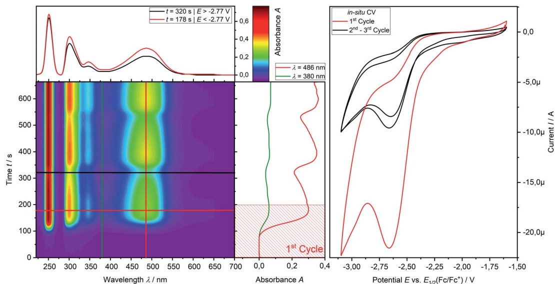
Fig. 3 Spectroelectrochemical UV-vis CV ( v = -15 \text{ mV s}^{-1} ) measurement of the reduction I of phosphine 3a (1.00 mM) in THF/0.1 M [ \text{Bu}_4\text{N} ][OTf] at a platinum grid electrode in double compartment cuvette cell. Left contour plot: relative UV-vis spectral changes during 3 cycles of CV; middle vertical plot: time dependent relative UV-vis absorbance; top left: projected relative UV-vis spectra after reduction in the 1 st CV cycle (red line) and after the 2 nd CV cycle (black line); right: in situ CV.
