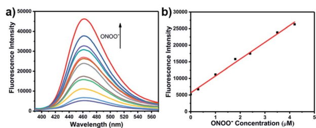
Fig. 2 (a) One-photon fluorescence spectra of LW-OTf (2.4 \mu\text{M} ) pre-incubated with O_2^{\cdot-} (5 \mu\text{M} ), followed by addition of ONOO^- (0–36 \mu\text{M} ). \lambda_{\text{ex/em}} = 360/461 nm. (b) Linear relationship between fluorescence intensity of LW-OTf (2.4 \mu\text{M} , pre-incubated with O_2^{\cdot-} (5 \mu\text{M} )) and concentration of ONOO^- (0–4.2 \mu\text{M} ). \lambda_{\text{ex/em}} = 360/461 nm. Note: O_2^{\cdot-} was prepared by dissolving KO_2 in DMSO, and was then added to LW-OTf (in DMSO), followed by addition of ONOO^- (in water). The mixture was diluted with PBS buffer (10 mM, pH 7.4) before each measurement. See ESI for detailed procedures.†
