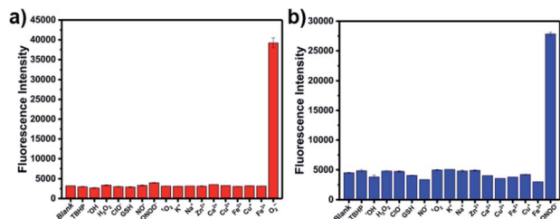
Fig. 3 (a) Red fluorescence response of LW-OTf (2.4 μM) to various reactive oxygen species/reactive nitrogen species or metals ions (100 μM TBHP, 100 μM ·OH, 10 mM H 2 O 2 , 100 μM NaClO, 10 μM GSH, 50 μM NO·, 25 μM ONOO - , 100 μM 1 O 2 , 10 mM K + , 10 mM Na + , 1 mM Zn 2+ , 1 mM Ca 2+ , 100 μM Cu 2+ , 100 μM Fe 2+ , 100 μM Cu + , 100 μM Fe 3+ , and 18 μM O 2 ·- ). λ ex/em = 675/710 nm. (b) One-photon blue fluorescence responses of probe LW-OTf (2.4 μM) to addition of O 2 ·- (5 μM) followed by addition of various reactive oxygen species/reactive nitrogen species or metal ions (100 μM TBHP, 100 μM ·OH, 10 mM H 2 O 2 , 100 μM NaClO, 10 μM GSH, 50 μM NO·, 100 μM 1 O 2 , 10 mM K + , 10 mM Na + , 1 mM Zn 2+ , 1 mM Ca 2+ , 100 μM Cu 2+ , 100 μM Fe 2+ , 100 μM Cu + , 100 μM Fe 3+ , and 4.2 μM ONOO - ). λ ex/em = 360/461 nm.
