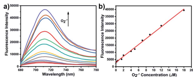
Fig. 1 (a) One-photon fluorescence spectra of LW-OTf (2.4 \mu\text{M} ) after addition of KO_2 (0–25 \mu\text{M} ). (b) Linear relationship between fluorescence intensity of LW-OTf (2.4 \mu\text{M} ) and concentration of O_2^{\cdot-} (0–18 \mu\text{M} ). \lambda_{\text{ex/em}} = 675/710 nm. Note: O_2^{\cdot-} was prepared by dissolving KO_2 in DMSO, and was then added to LW-OTf (in DMSO). The mixture was diluted with PBS buffer (10 mM, pH 7.4) before each measurement. See ESI for detailed procedures.†
