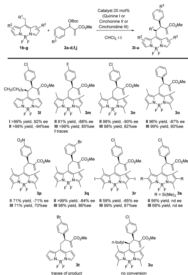
Scheme 2 Scope of the reaction of BODIPY 1b–g with MBH 2a–d, f, j . In a closed vial were added the organic catalyst quinine, cinchonine or cinchonidine (20 mol%), the BODIPY (0.05 mmol, 1 equiv.), the Morita–Baylis–Hillman carbonate (2 equiv.), and chloroform (1 ml) and stirred at rt for 2–10 days, monitored by 1 H-NMR. The crude was purified by flash column chromatography ( n -hexane/EtOAc) to obtain the desired product. The regioselectivity and diastereoselectivity were determined by 1 H-NMR analysis of the crude reaction mixture (in all the examples, only one diastereomer was detected). The ee was determined by chiral HPLC.
