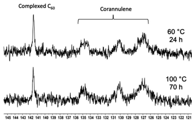
Fig. 8 ^{13}\text{C} NMR spectra showing the \text{C}_{60} signal in the polymer nanoparticle core after heating at 60 (top) and 100 ^{\circ}\text{C} (bottom) for 24 and 70 hours, respectively.
