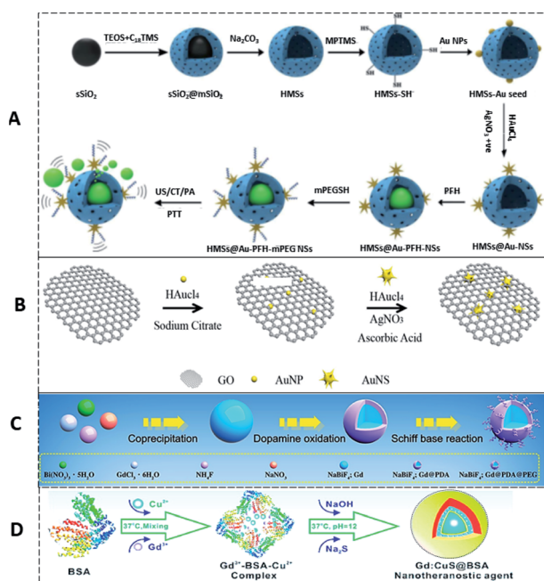
Fig. 8 (A) Schematic illustration of the synthesis of HMSs, HMSs@Au Ns, and HAPPs, 145 reproduced from ref. 145 with permission from the American Chemical Society, copyright 2017. (B) rGO/Au Ns nano-composite, 147 reproduced from ref. 147 with permission from the American Chemical Society, copyright 2019. (C) NaBiF 4 :Gd-PDA-PEG NPs, 150 reproduced from ref. 150 with permission from the American Chemical Society, copyright 2020. (D) Gd:CuS@BSA NPs, 151 reproduced from ref. 151 with permission from the American Chemical Society, copyright 2016.
