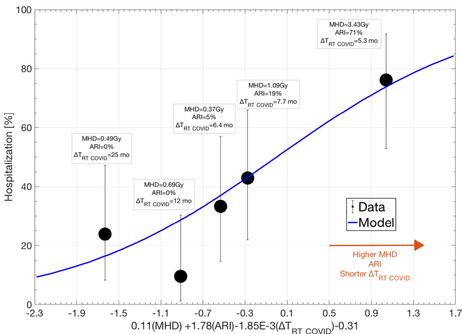
Fig. 2. The dose–response curve for the multivariate hospitalization model in the validation data. The model included ARI, MHD and ΔT RT COVID . The solid blue line is the model; black quintiles represent data (error bars: 95% exact binomial confidence intervals). Above each quintile, the population average MHD and ΔT RT COVID are given along with the ARI rate.
