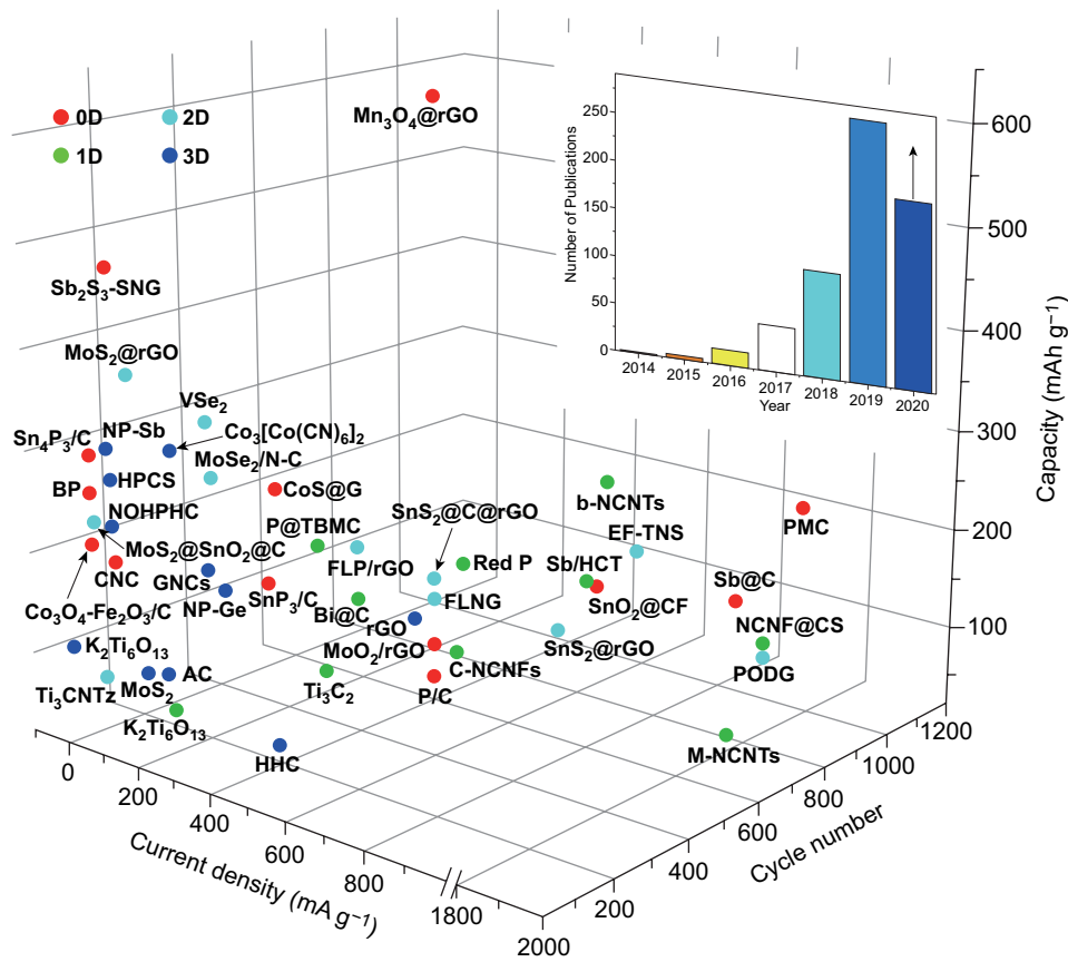
Fig. 1 Cycle capacity of various PIBs anode materials reported recently. Sb 2 S 3 -SNG [38]; Co 3 O 4 -Fe 2 O 3 /C [39]; black phosphorus=BP [33]; Sn 4 P 3 /C [40]; CoS@G [41]; CNC [42]; PMC [43]; Sb@C [44]; P/C [45]; MoO 2 /rGO hollow sphere composites=MoO 2 /rGO [46]; Mn 3 O 4 @rGO [47]; SnP 3 /C [48]; SnO 2 nanoparticles anchored on carbon foam=SnO 2 @CF [49]; P@TBMC [50]; NCNF@CS [51]; alkalinized Ti 3 C 2 MXene nanoribbons=Ti 3 C 2 [52]; chitin-derived NCNFs=C-NCNFs [53]; bamboo-like NCNTs=b-NCNTs [54]; MOF-derived NCNTs=M-NCNTs [55]; red P [56]; segment-like Sb nanorod encapsulated in hollow carbon tube=Sb/HCT [57]; K 2 Ti 6 O 13 [58]; Bi@C [59]; Ti 3 CNTz [60]; MoS 2 @rGO [61]; MoS 2 @SnO 2 @C [62]; graphene-like VSe 2 nanosheets=VSe 2 [63]; Few-layered SnS 2 nanosheets supported on rGO=SnS 2 /rGO [64]; FLNG [65]; PODG [66]; MoSe 2 /N-C [67]; EF-TNS [68]; FLP/rGO [69]; MoS 2 [70]; K 2 Ti 6 O 13 [71]; NP-Sb [72]; NP-Ge [73]; activated carbon=AC [74]; Co 3 [Co(CN) 6 ] 2 [75]; HPCS [76]; N/O co-doped mesoporous carbon octahedrons=NOHPhC [77]; rGO aerogel=rGO [78]; GNCs [79]; honeycomb hard carbon=HHC [80]. And the inset about number of articles obtained from Web of Science on PIBs anode materials and based on the corresponding Topic about potassium ion battery, potassium ion storage, potassium storage, and anode (accessed: July 1, 2020)
