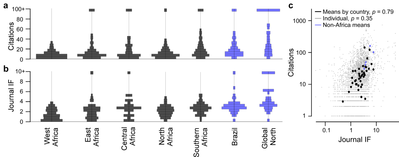
Fig. 2 Citations and journal impact factors. a, b Area-normalised histograms of citations ( a ) and the publishing journal's impact factor (IF, b ) of all papers from different African and non-African regions, as indicated. In each case, all citations above \geq 95 , and IF above \geq 9.5 were allocated to a single bin (top). c Citations plotted against IF for every paper in the database (small grey dots), and for means by country (large dots), as indicated. Linear correlation coefficients as indicated. Source data are provided as a Source Data file.
