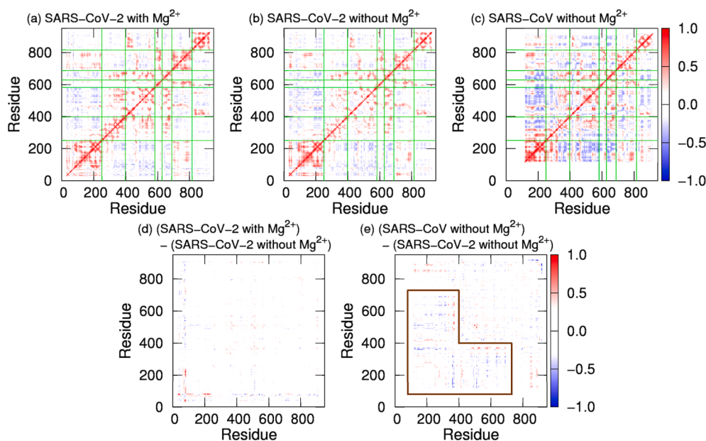
Fig. 7. DCC for (a) the SARS-CoV-2 nsp12 with Mg^{2+} , (b) that without Mg^{2+} , and (c) the SARS-CoV nsp12. (d) Differences between DCCs for the SARS-CoV-2 nsp12 with Mg^{2+} and those for the SARS-CoV-2 nsp12 without Mg^{2+} . (e) Differences between DCCs for the SARS-CoV nsp12 and those for the SARS-CoV-2 nsp12 without Mg^{2+} . The green lines show the borders between the domains in nsp12. Residues that have large differences are surrounded by the brown lines.
