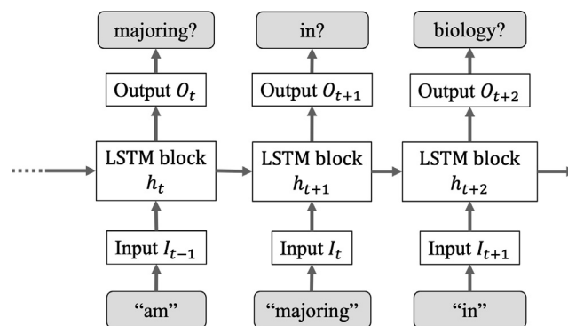
Fig. 4. Graphical representation of a forward LSTM. Input I_t shows the embedding of the t -th word w_t , and the output O_t is transformed to a probability using a softmax function. For example, if w_t is “majoring”, the model is trained to increase the possibility that “majoring” is output from O_t , which is calculated from words up to w_{t-1} , “am”.
