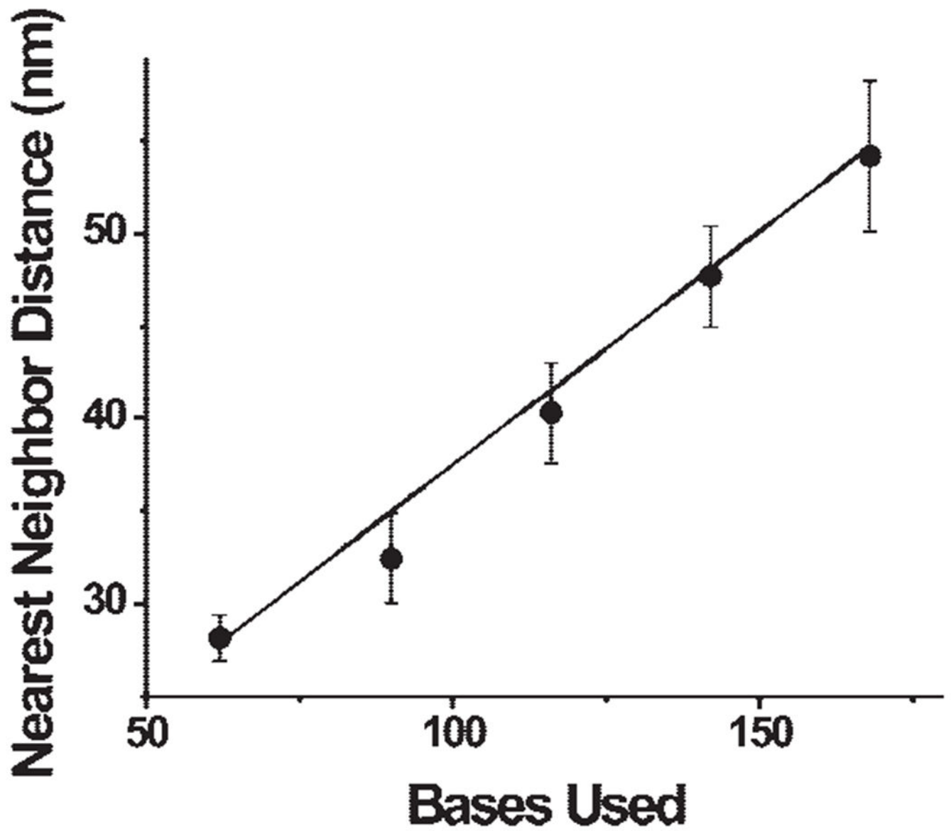
Figure 3. Interparticle spacing as a function of total DNA length. A plot of the gold nearest neighbor distances as a function of the total number of bases used to separate them.
