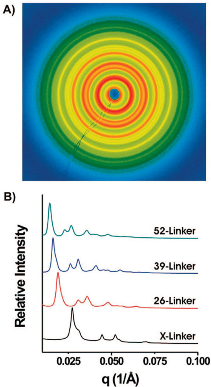
Figure 1. 2-Dimensional and 1-Dimensional SAXS data. (A) 2-D data collected for the N=39 linker system displayed in false colors. (B) 1-D line profiles of the 2-D data taken for the X-linker, N=26 , 39, and 52 systems demonstrating that the q^* peak shifts to smaller values of q with increasing linker length. The 1-Dimensional data for the N=13 bp linker was not included in part B, as this structure could not be annealed at 35^\circ\text{C} due to the low melting temperature of the A13/T13 duplex region. When N=13 aggregates were formed at room temperature
