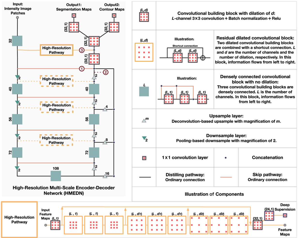
Fig. 2. Illustration of the structure of our proposed high-resolution multi-scale encoder-decoder network (HMEDN). The input is a set of intensity image patches and the outputs are segmentation and contour probability maps. Rectangles and triangles represent operations in the network. Three kinds of pathways, i.e., skip connection (pathway ①), distilling pathway (pathway ②) and high-resolution pathway (pathway ③) connect all kinds of operations and form the network.
