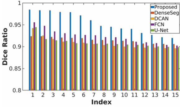
(a) Prostate: The top 15.
