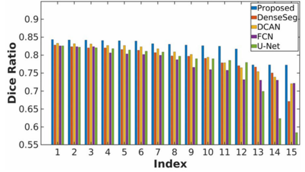
(b) Prostate: The Worst 15.
