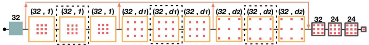
Fig. 3. Illustration of the dilated convolutional network.
