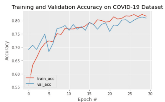
(e) Accuracy curve of VGG16
