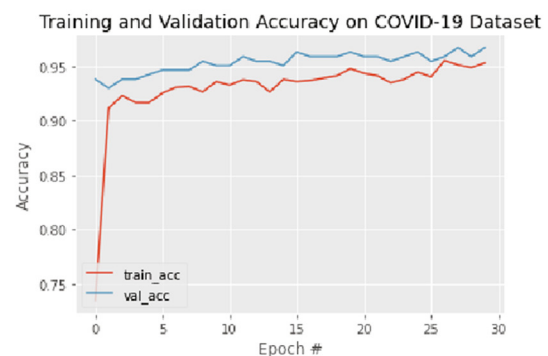
(e) Accuracy curve of VGG16
