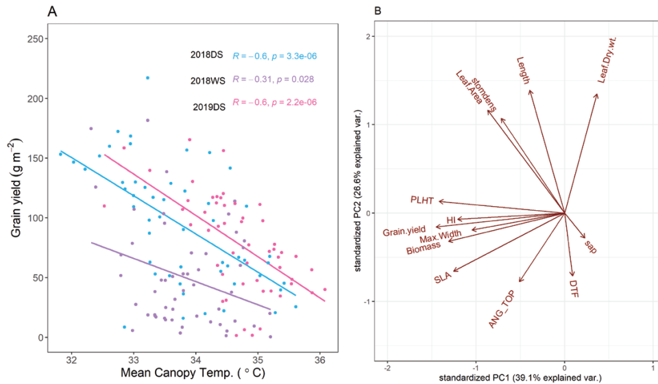
Fig. 5. Effect of canopy temperature on grain yield in rice and principal component analysis of traits in the IRRI trials. (A) Linear regressions between grain yield and mean canopy temperature across five, 14, and 18 measurement dates in 2018DS, 2018WS, and 2019DS, respectively. Each point represents one experimental plot, and genotypes are listed in Supplementary Table S2 . DS, dry season; WS, wet season. (B) Principal component analysis of leaf, root, and agronomic traits measured across all IRRI trials. Mean canopy temperature was only measured in the 2018DS–2019DS stress treatments and is not included. Length, flag-leaf length; Leaf.Dry.wt: flag-leaf dry weight; sap, xylem sap bleeding rate; DTF, days to flowering; ANG_Top, root crown top angle; SLA, specific leaf area of the flag leaf; Biomass, straw biomass at harvest; Max.Width, maximum flag-leaf width; Grain.yield, grain yield at harvest; HI, harvest index; PLHT, plant height at flowering; Leaf.Area, flag-leaf area; stomdens, stomatal density of the penultimate leaf on the plant.
