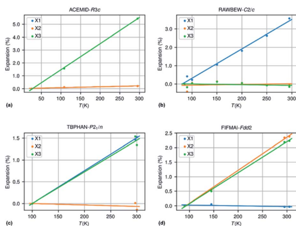
Fig. 6 (a) ACEMID – acetamide; IAC = 0.96 (three different studies); (b) RAWBEW – biguanidinium bis(dinitramide); IAC = 0.94 (three different studies); (c) TBPAN – tetrabromophthalic anhydride; IAC = -0.91 ; (2 different studies); (d) FIFMAI – 2-biphenylol IAC = -0.91 (1 study).
