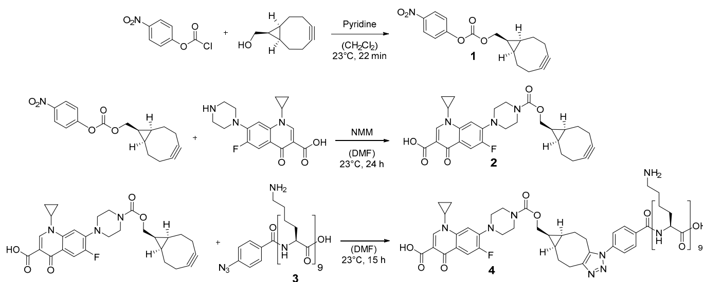
Figure 1. Reaction scheme for the preparation of ciprofloxacin conjugated to a poly-L-lysine sequence which can be used as linker.
