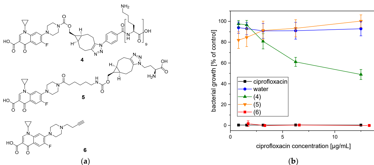
Figure 6. Bacterial growth in the presence of ciprofloxacin modifications. (a) Chemical structures of the ciprofloxacin modifications 4 , 5 , and 6 . (b) Percentage growth of S. aureus (mean \pm SD) in the presence of different concentrations of ciprofloxacin modifications ( 4 , 5 , 6 ), unmodified ciprofloxacin, or water.
